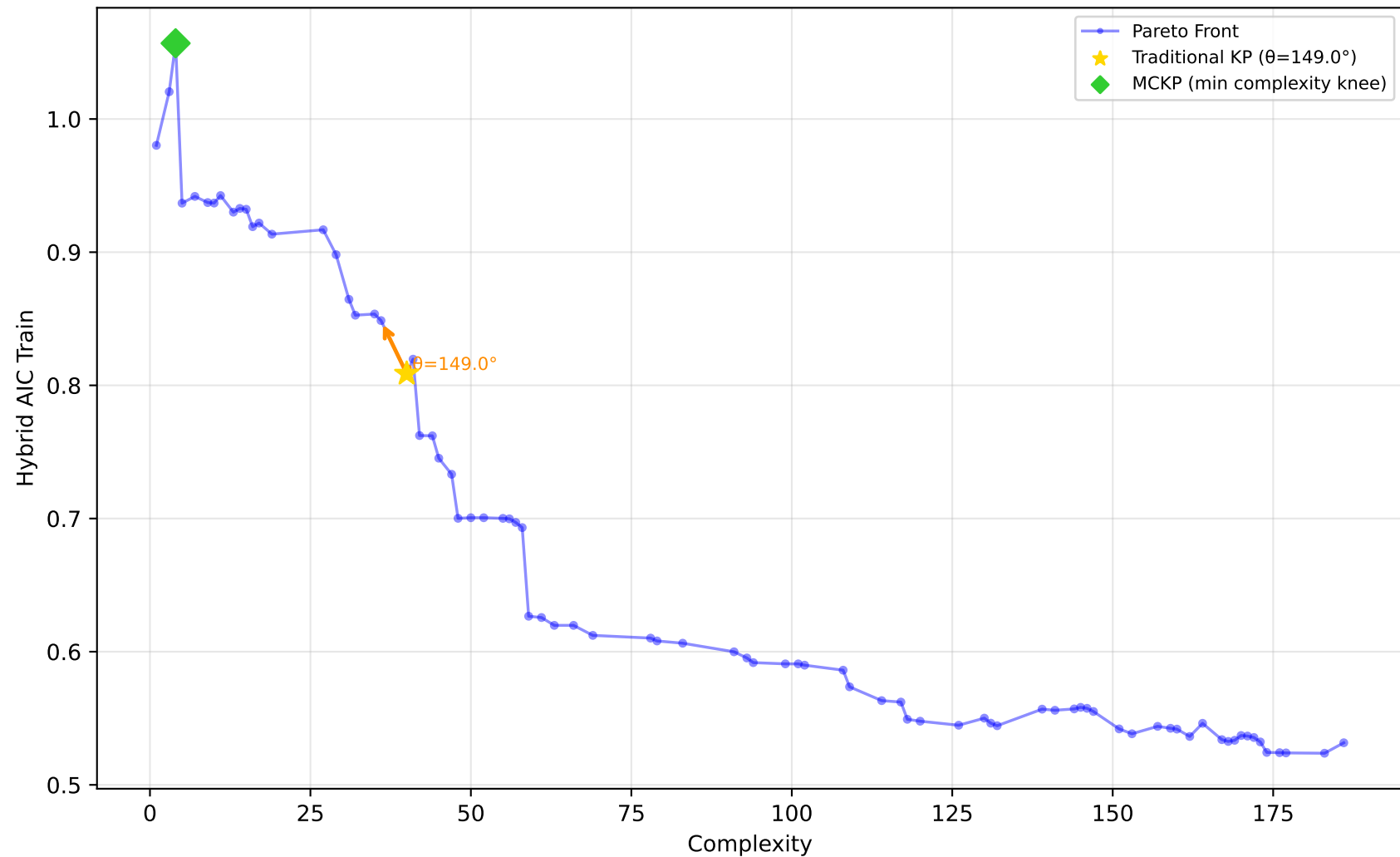
1096_FacultySalaries - Run 18 - SVP - Hybrid AIC Train \lambda_1=1.00, \lambda_2=0.00, \lambda_3=0.00 | Difficulty: 1.00 | Method: hmr
