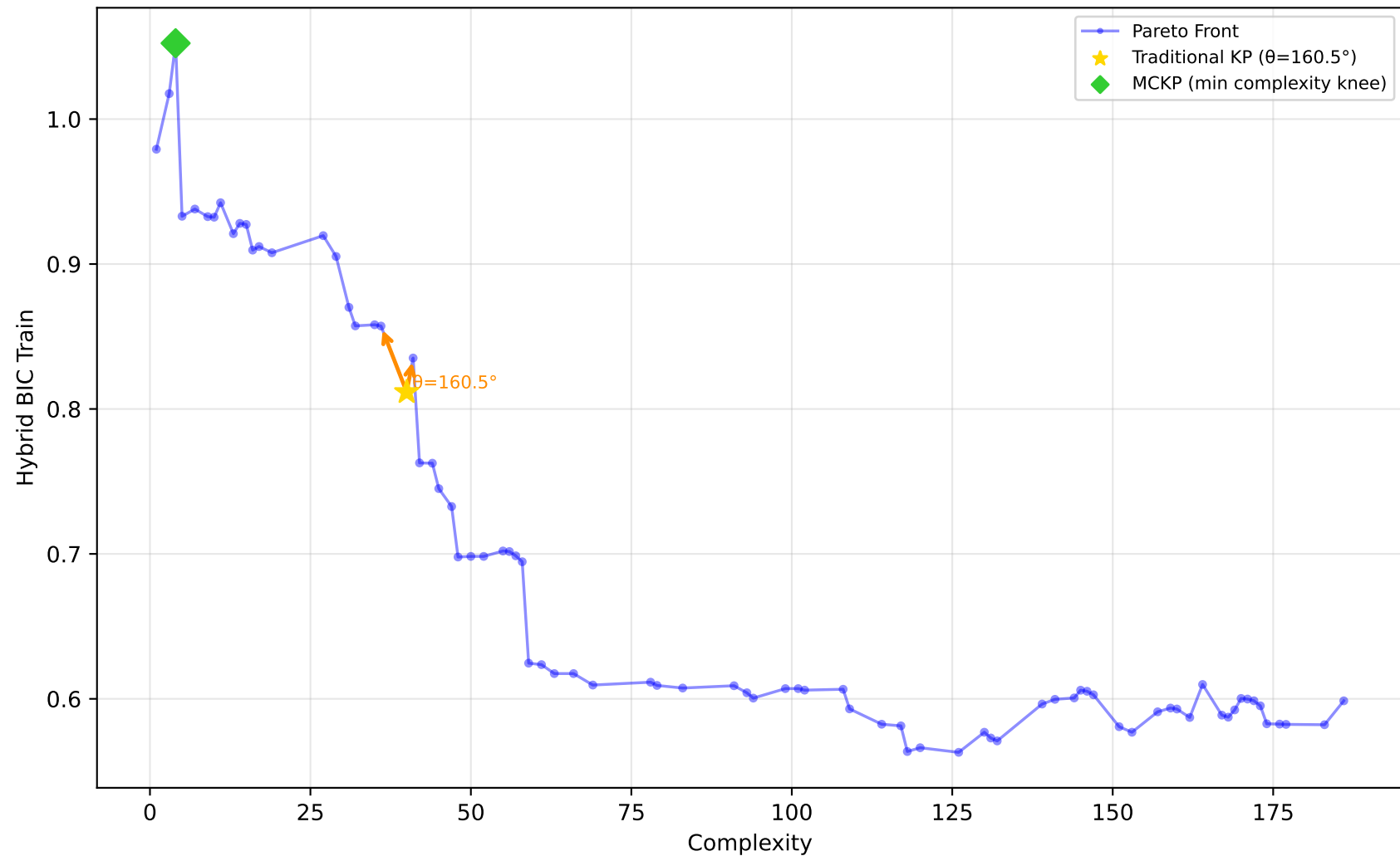
1096_FacultySalaries - Run 18 - SVP - Hybrid BIC Train \lambda_1=1.00 , \lambda_2=0.00 , \lambda_3=0.00 | Difficulty: 1.00 | Method: hmr
