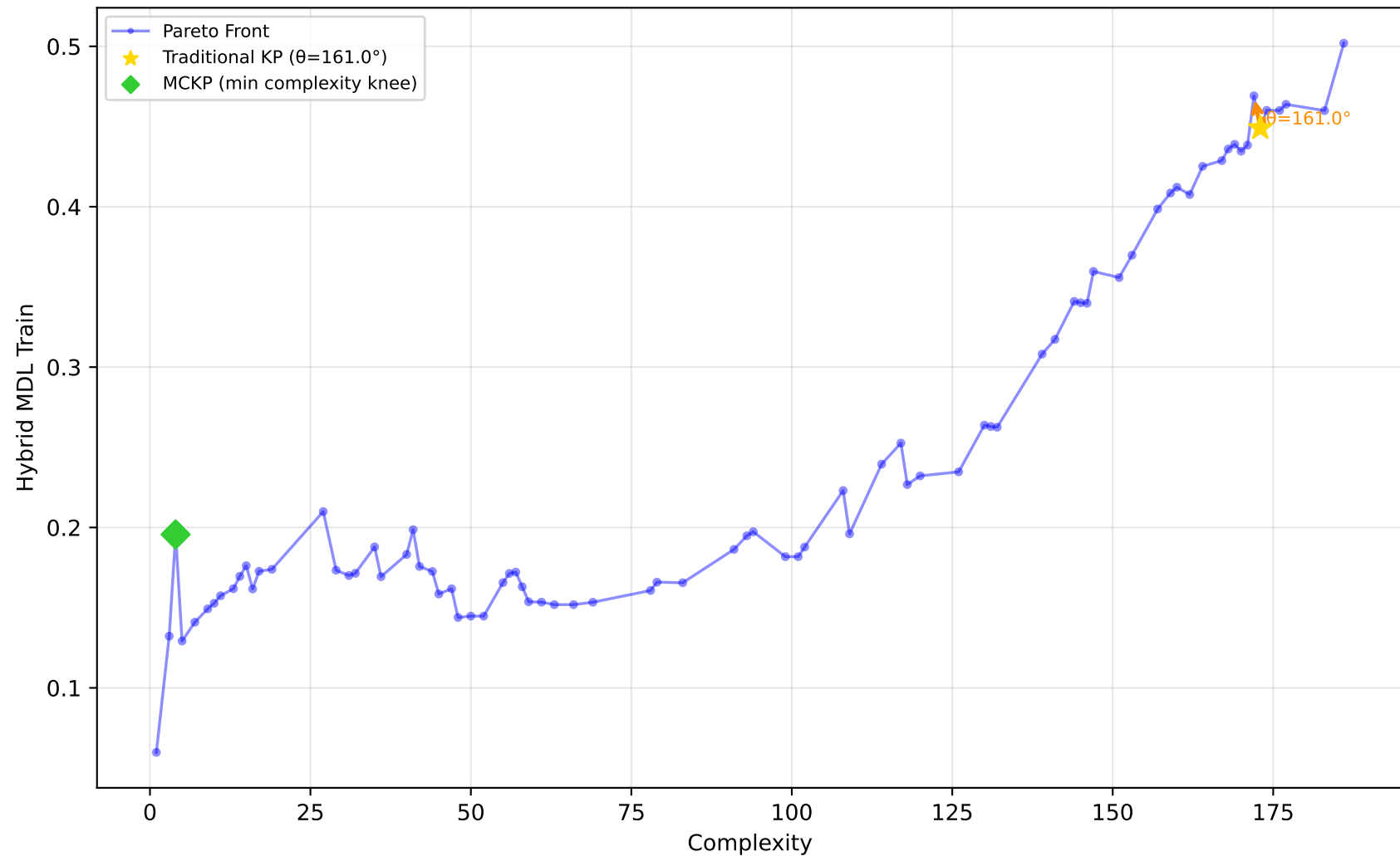
1096_FacultySalaries - Run 18 - SVP - Hybrid MDL Train \lambda_1=1.00, \lambda_2=0.00, \lambda_3=0.00 | Difficulty: 1.00 | Method: hmr
