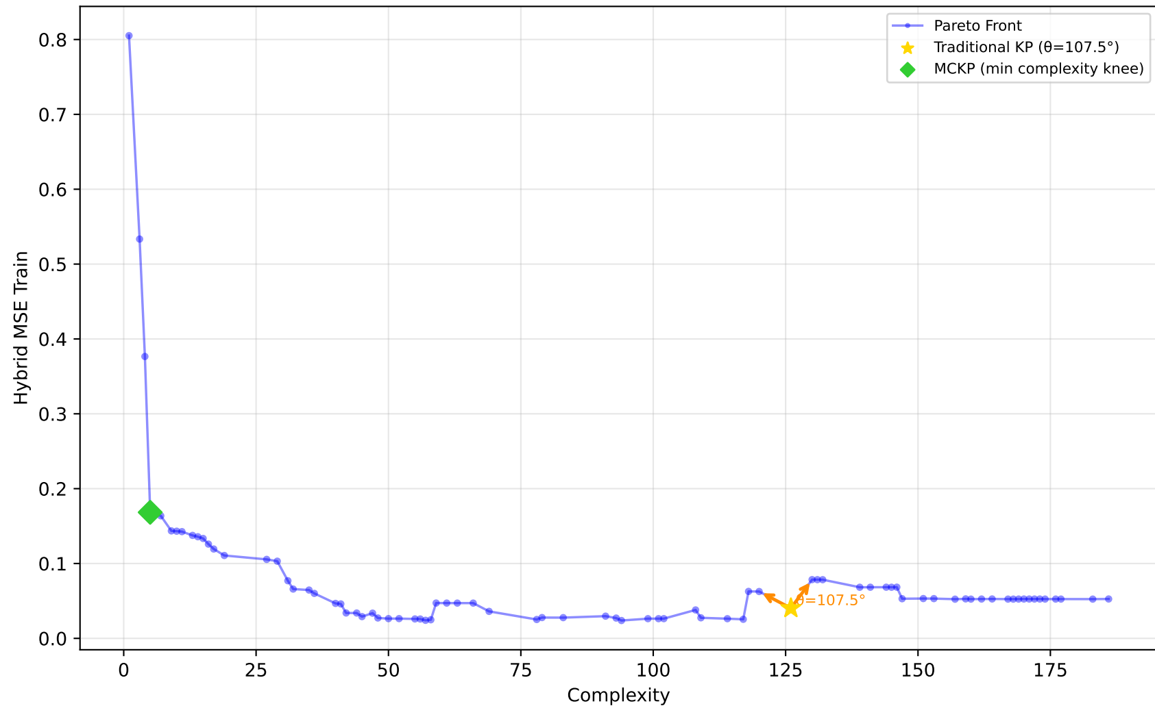
1096_FacultySalaries - Run 18 - SVP - Hybrid MSE Train \lambda_1=0.00, \lambda_2=0.90, \lambda_3=0.00 | Difficulty: 1.00 | Method: hmr
