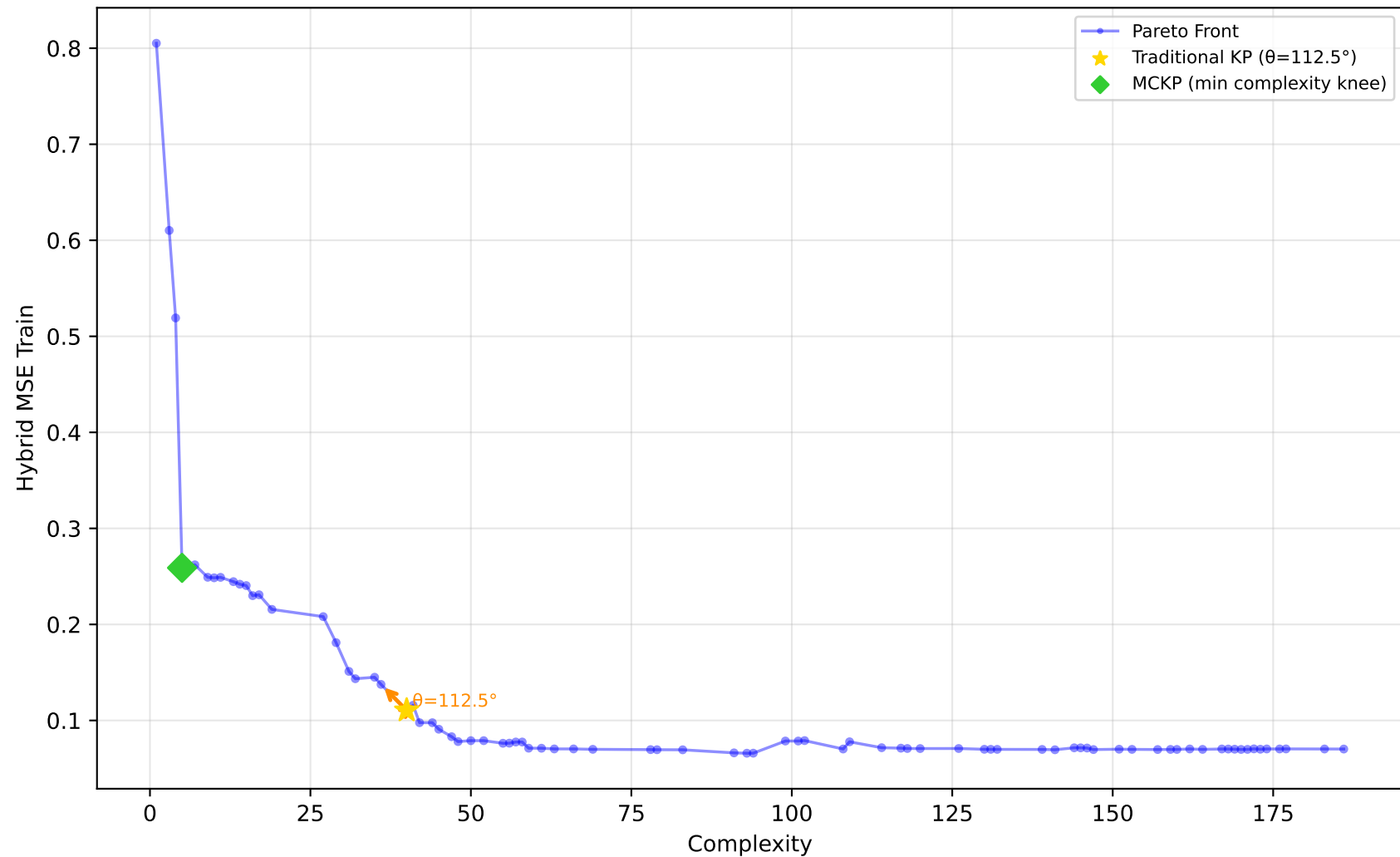
1096_FacultySalaries - Run 18 - SVP - Hybrid MSE Train \lambda_1=1.00, \lambda_2=0.00, \lambda_3=0.00 | Difficulty: 1.00 | Method: hmr
