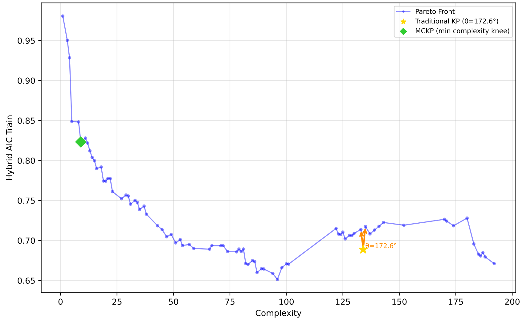
1096_FacultySalaries - Run 19 - MVP - Hybrid AIC Train \lambda_1=0.10 , \lambda_2=0.00 , \lambda_3=0.00 | Difficulty: 1.00 | Method: hmr
