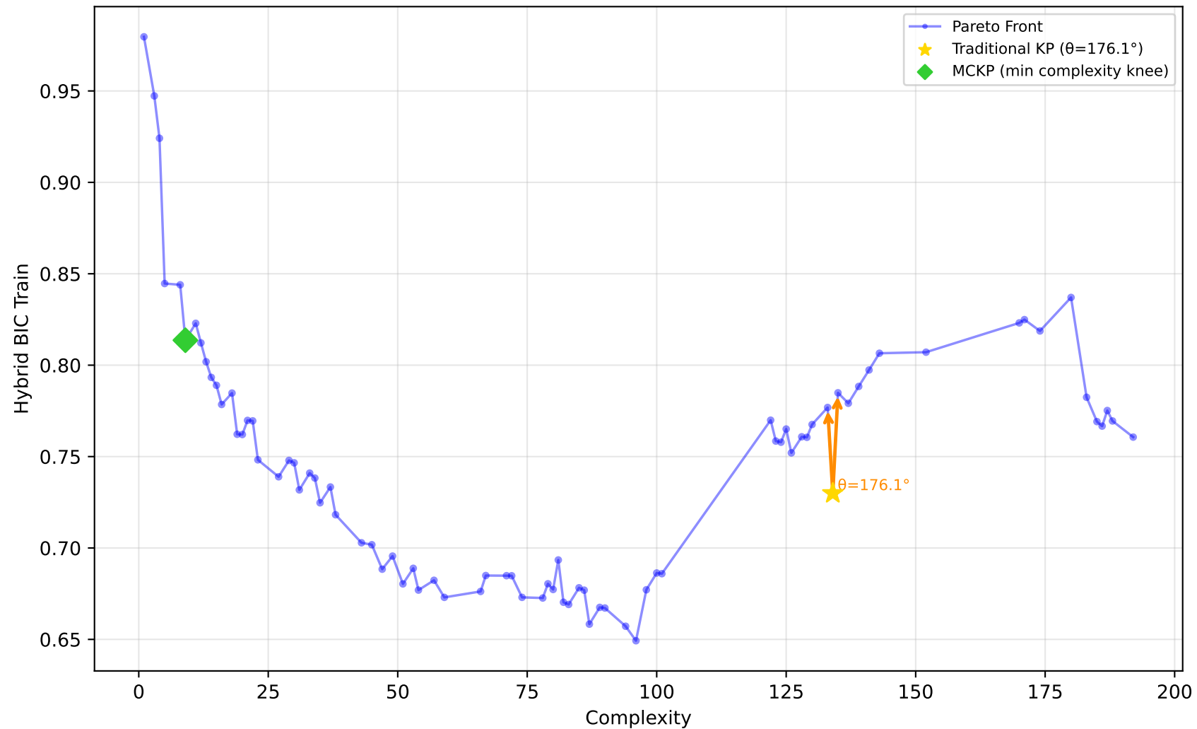
1096_FacultySalaries - Run 19 - MVP - Hybrid BIC Train \lambda_1=0.10 , \lambda_2=0.00 , \lambda_3=0.00 | Difficulty: 1.00 | Method: hmr
