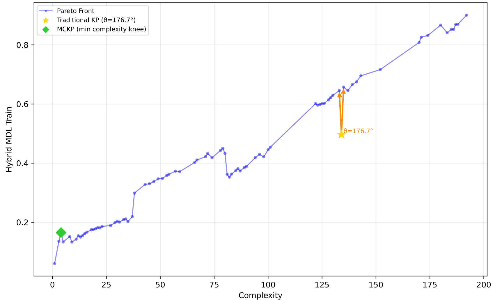
1096_FacultySalaries - Run 19 - MVP - Hybrid MDL Train \lambda_1=1.00, \lambda_2=0.00, \lambda_3=0.00 | Difficulty: 1.00 | Method: hmr
