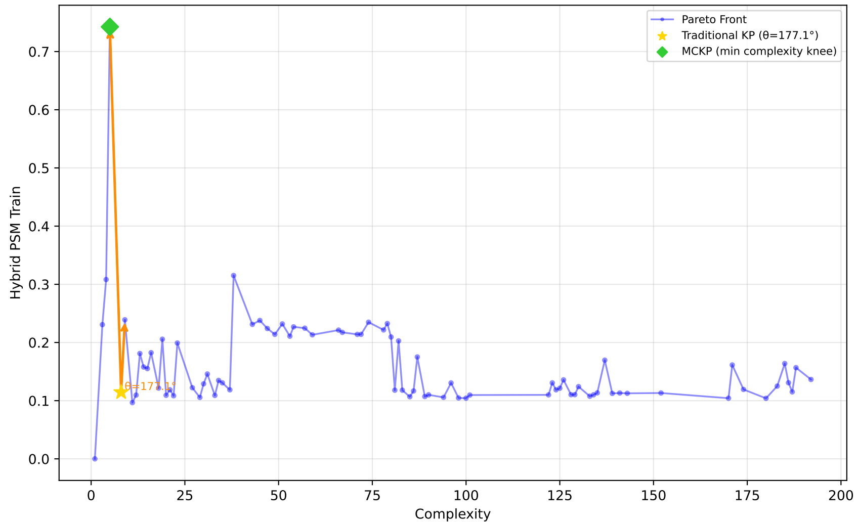
1096_FacultySalaries - Run 19 - MVP - Hybrid PSM Train \lambda_1=1.00, \lambda_2=0.00, \lambda_3=0.00 | Difficulty: 1.00 | Method: hmr
