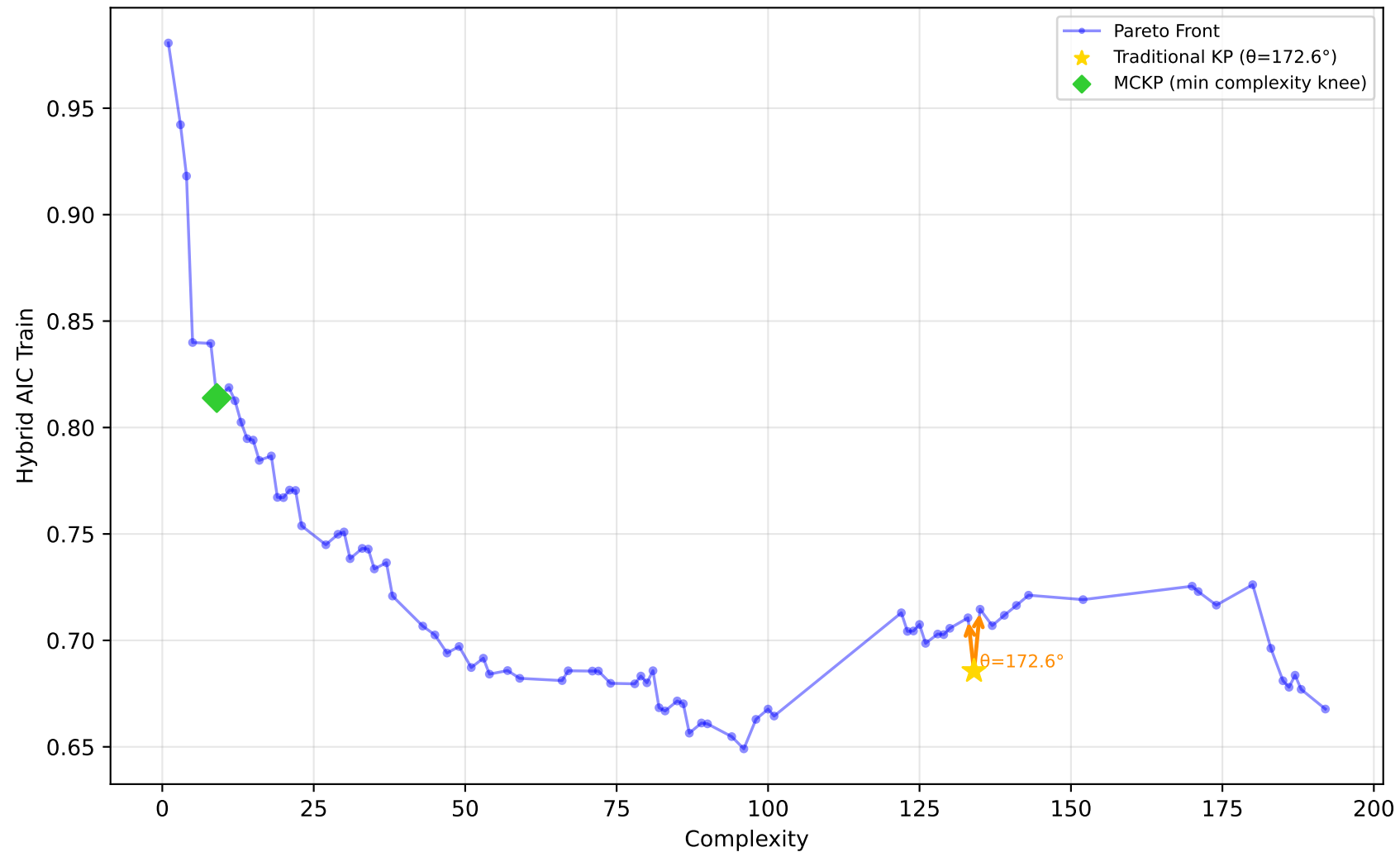
1096_FacultySalaries - Run 19 - SVP - Hybrid AIC Train \lambda_1=0.00 , \lambda_2=0.90 , \lambda_3=0.00 | Difficulty: 1.00 | Method: hmr
