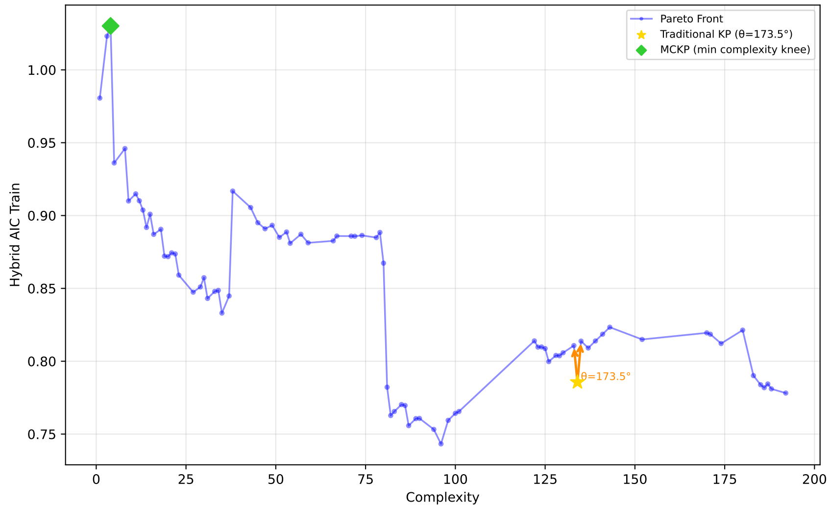
1096_FacultySalaries - Run 19 - SVP - Hybrid AIC Train \lambda_1=1.00 , \lambda_2=0.00 , \lambda_3=0.00 | Difficulty: 1.00 | Method: hmr
