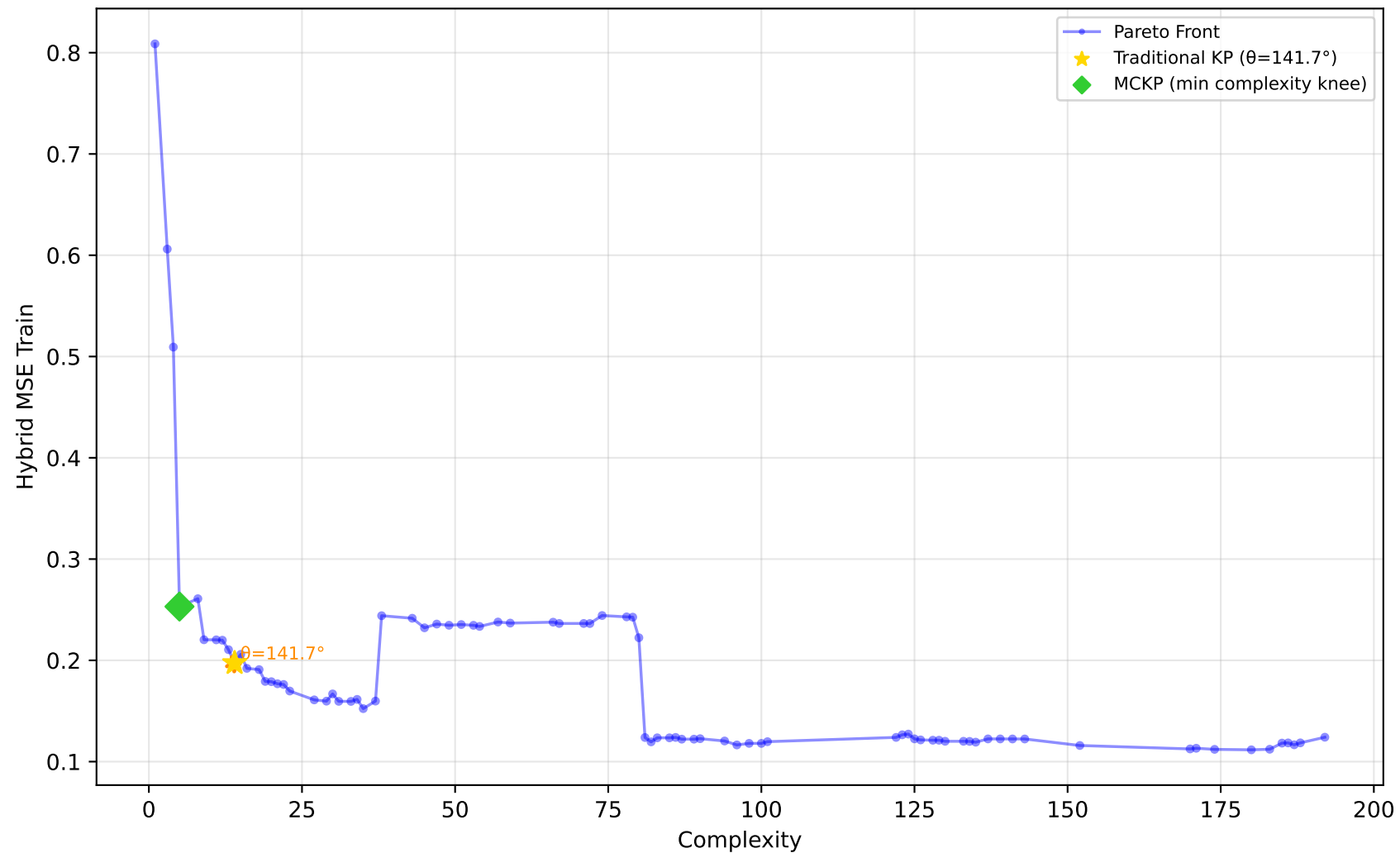
1096_FacultySalaries - Run 19 - SVP - Hybrid MSE Train \lambda_1=1.00, \lambda_2=0.00, \lambda_3=0.00 | Difficulty: 1.00 | Method: hmr
