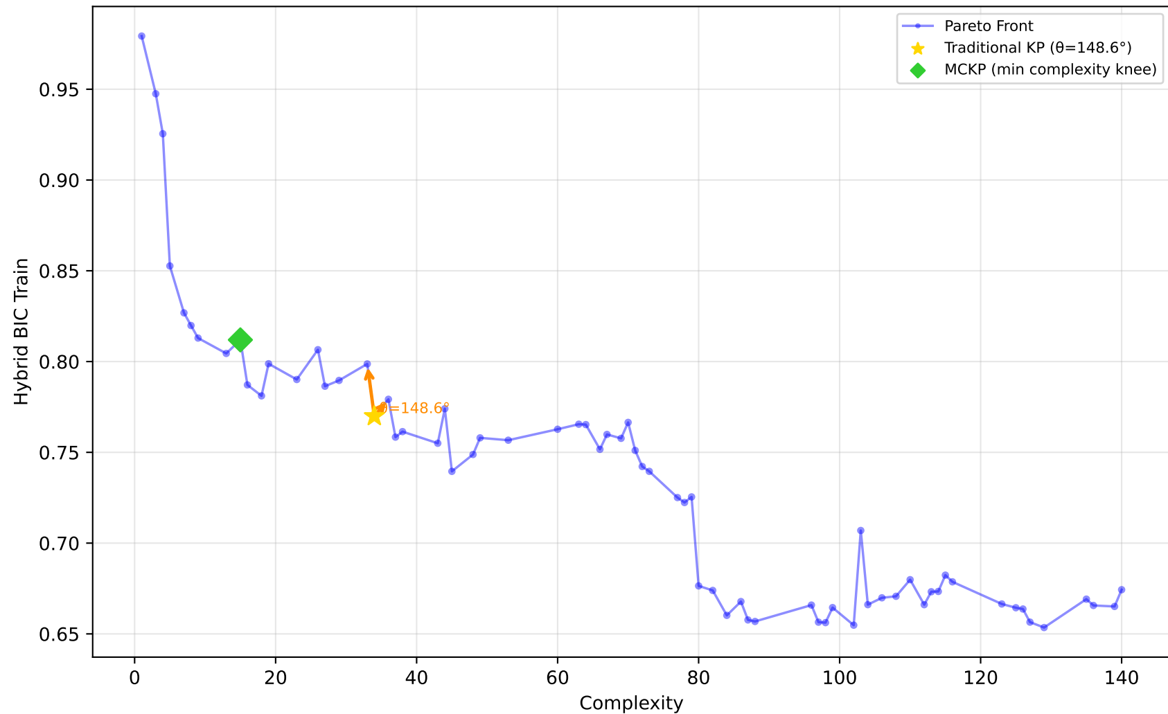
1096_FacultySalaries - Run 1 - MVP - Hybrid BIC Train \lambda_1=0.10, \lambda_2=0.00, \lambda_3=0.00 | Difficulty: 0.47 | Method: mckp
