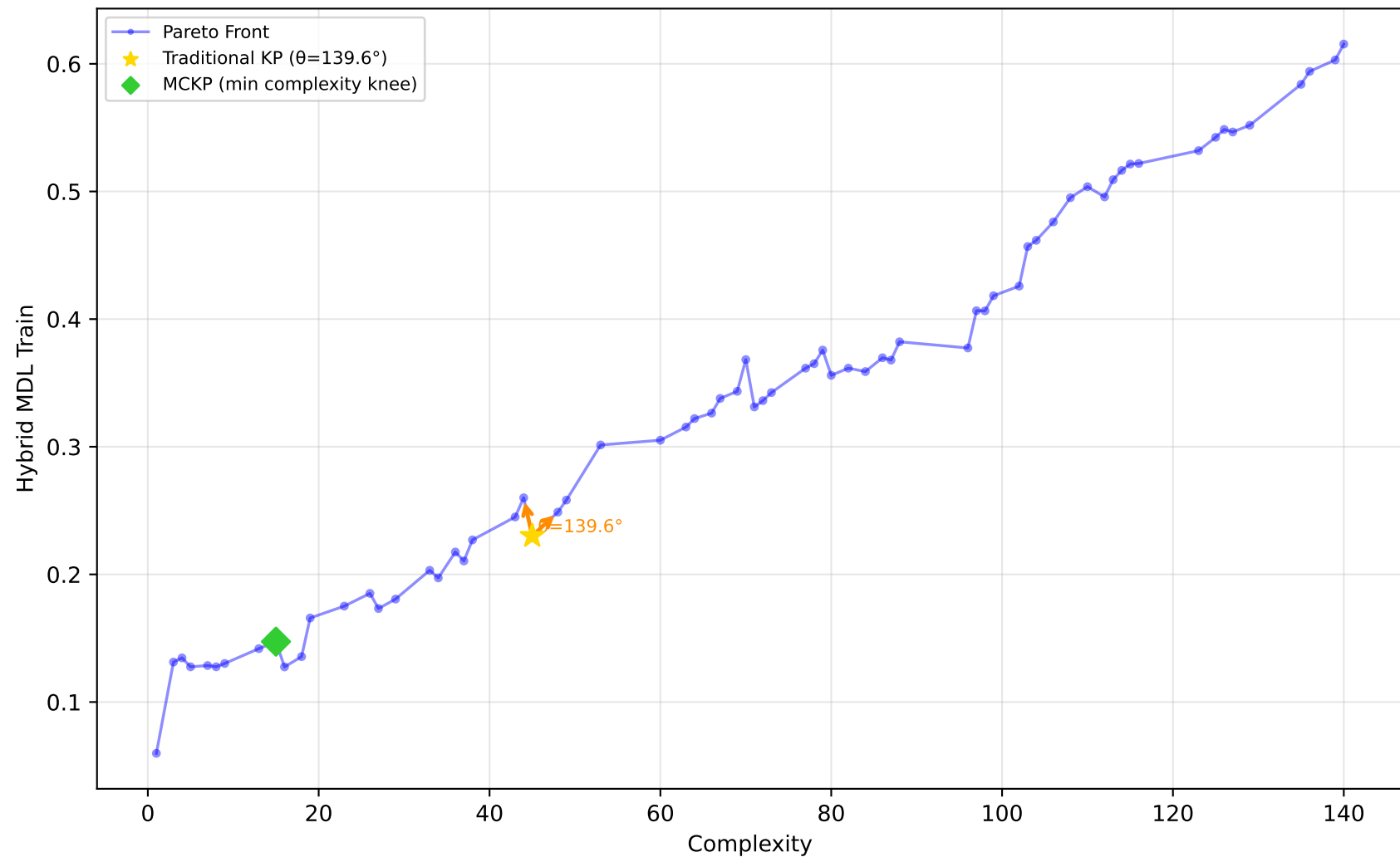
1096_FacultySalaries - Run 1 - MVP - Hybrid MDL Train \lambda_1=1.00, \lambda_2=0.00, \lambda_3=0.00 | Difficulty: 0.47 | Method: mckp
