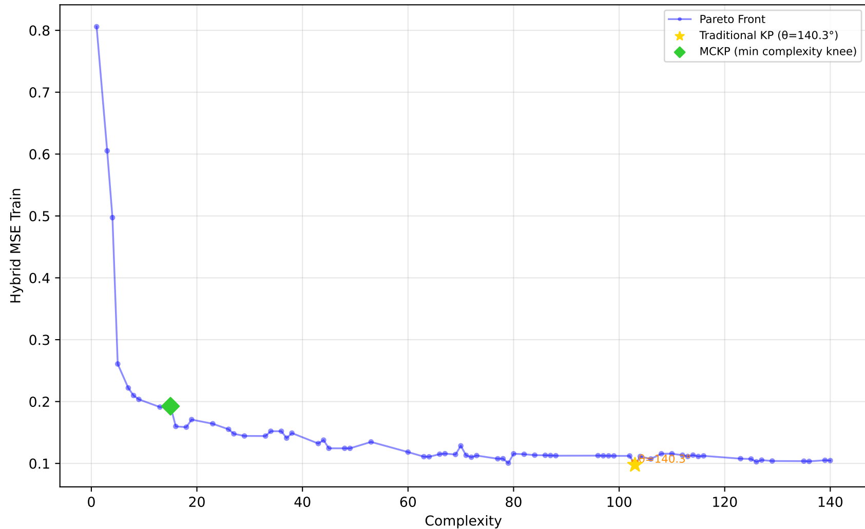
1096_FacultySalaries - Run 1 - MVP - Hybrid MSE Train \lambda_1=1.00, \lambda_2=0.00, \lambda_3=0.00 | Difficulty: 0.47 | Method: mckp
