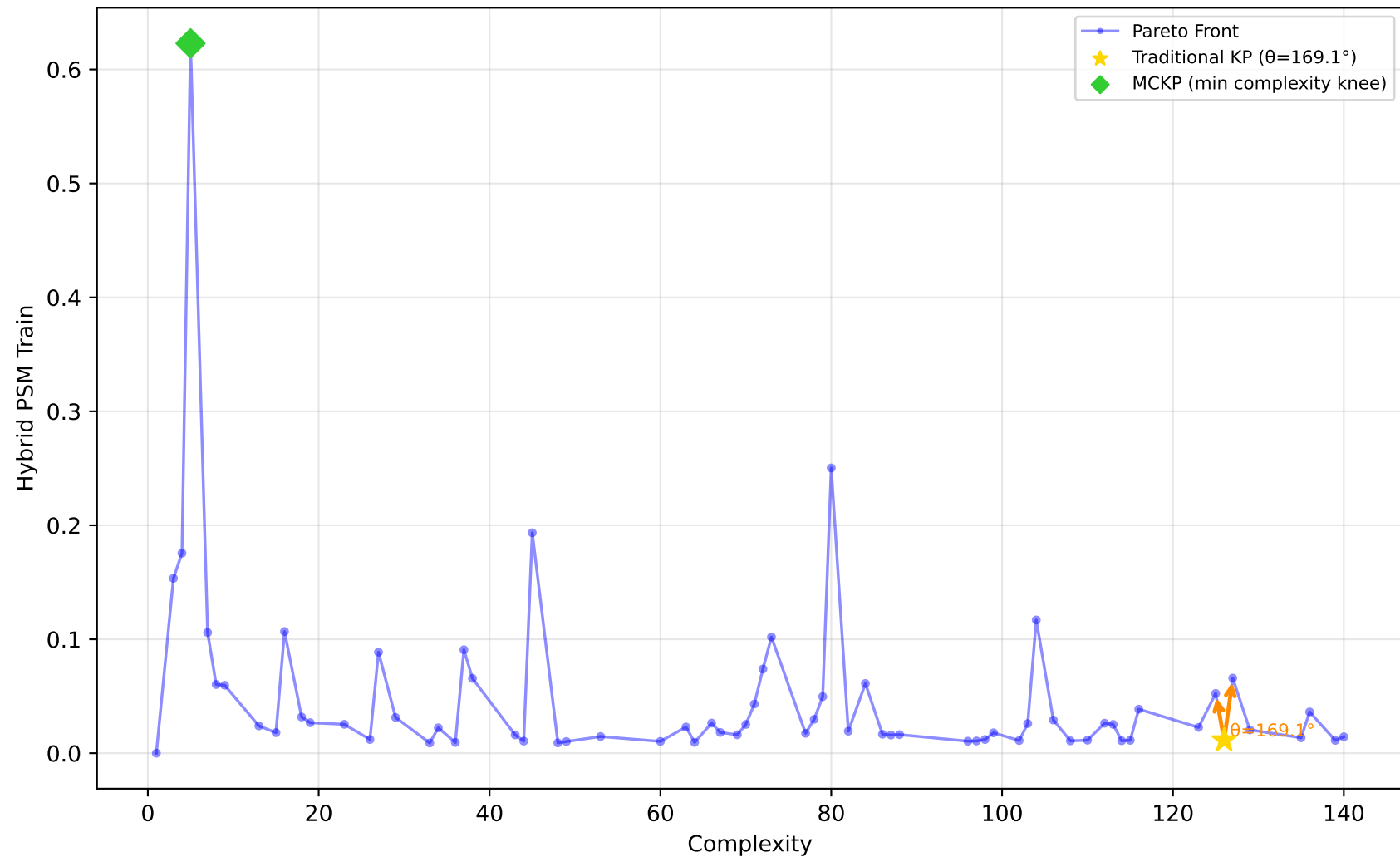
1096_FacultySalaries - Run 1 - MVP - Hybrid PSM Train \lambda_1=0.10, \lambda_2=0.00, \lambda_3=0.00 | Difficulty: 0.47 | Method: mckp
