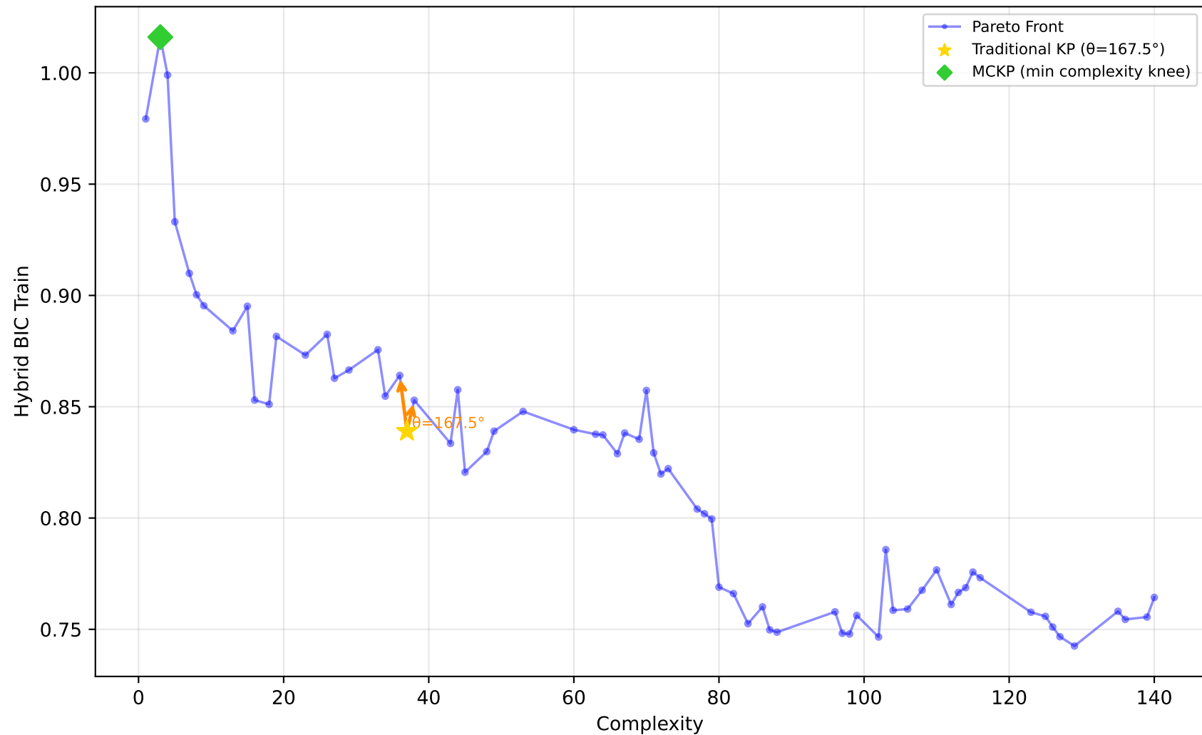
1096_FacultySalaries - Run 1 - SVP - Hybrid BIC Train \lambda_1=1.00, \lambda_2=0.00, \lambda_3=0.00 | Difficulty: 0.47 | Method: mckp
