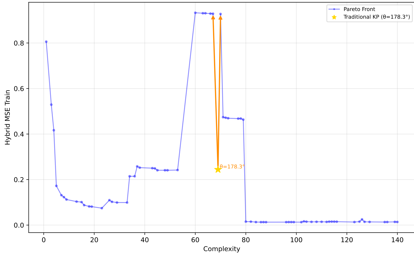
1096_FacultySalaries - Run 1 - SVP - Hybrid MSE Train \lambda_1=0.00, \lambda_2=0.90, \lambda_3=0.00 | Difficulty: 0.47 | Method: mckp
