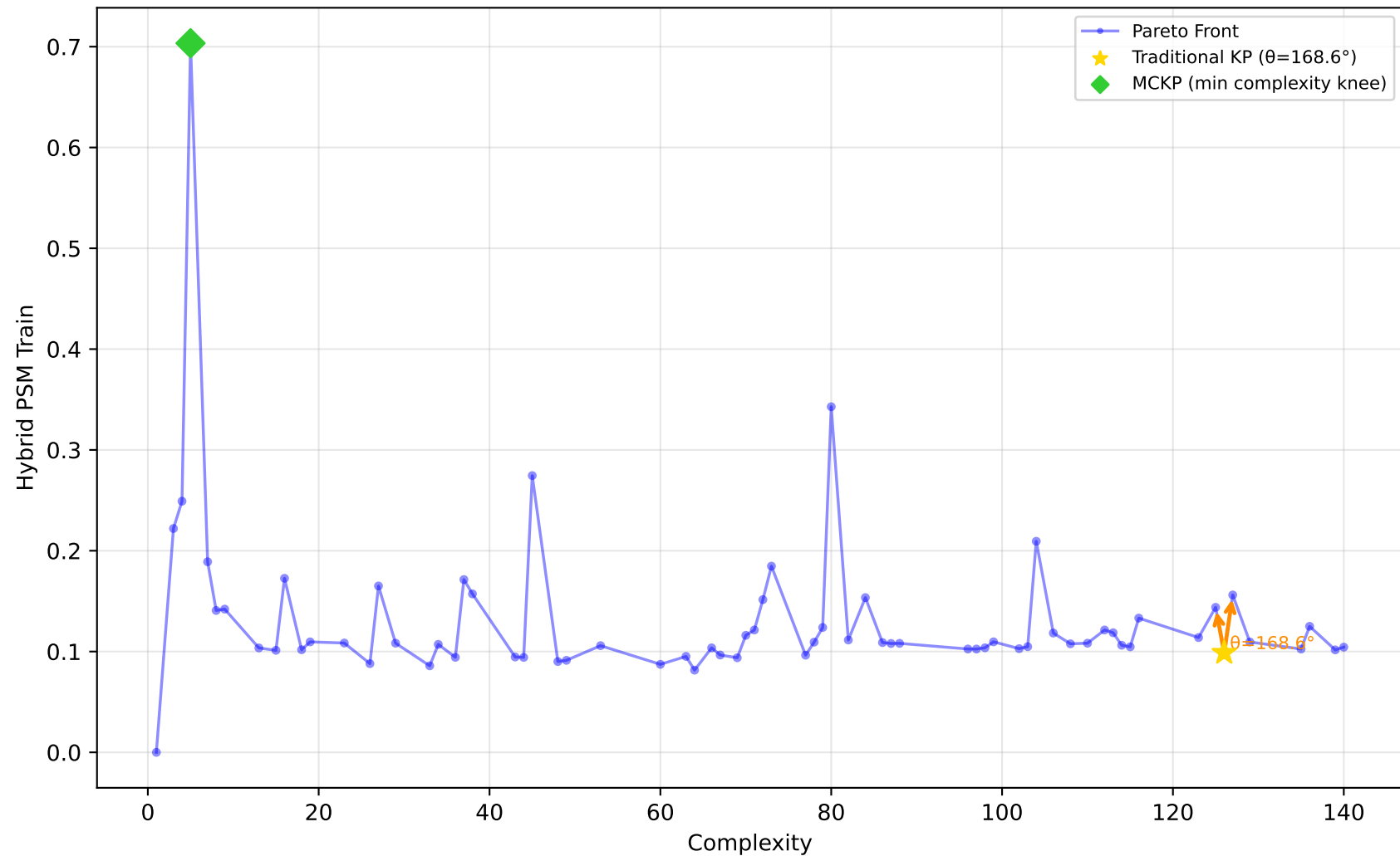
1096_FacultySalaries - Run 1 - SVP - Hybrid PSM Train \lambda_1=1.00, \lambda_2=0.00, \lambda_3=0.00 | Difficulty: 0.47 | Method: mckp
