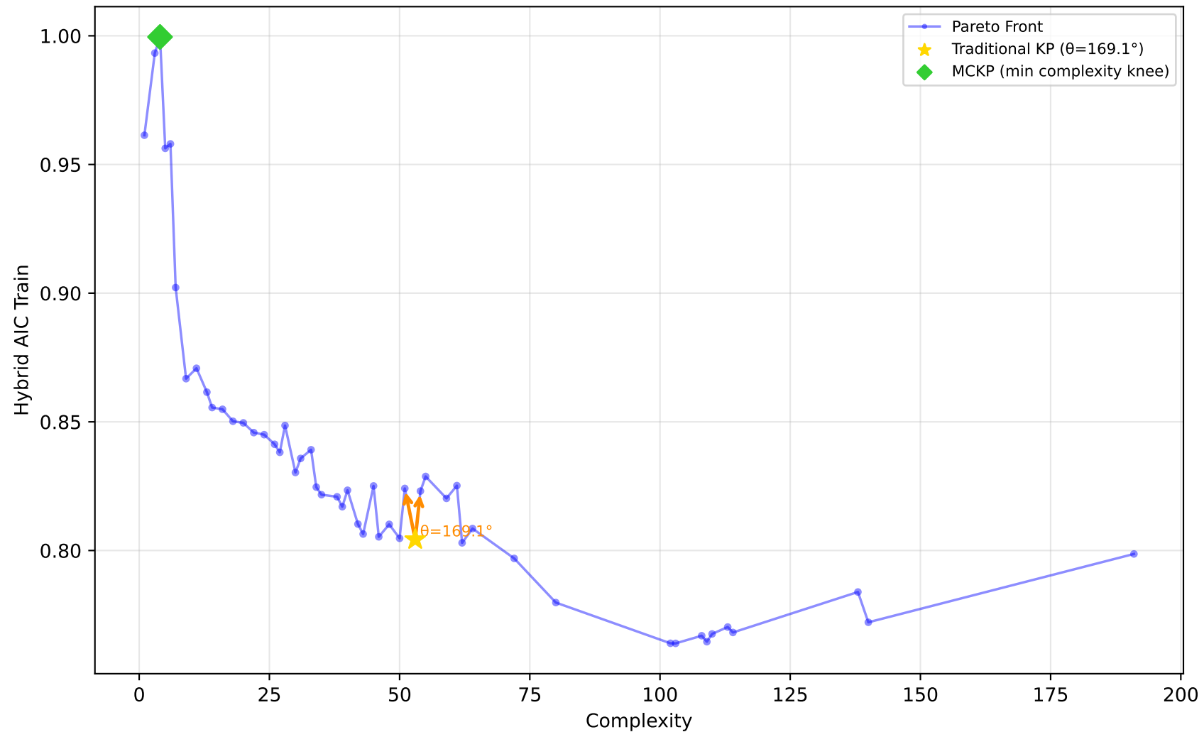
1096_FacultySalaries - Run 20 - MVP - Hybrid AIC Train \lambda_1=1.00, \lambda_2=0.00, \lambda_3=0.00 | Difficulty: 0.41 | Method: mckp
