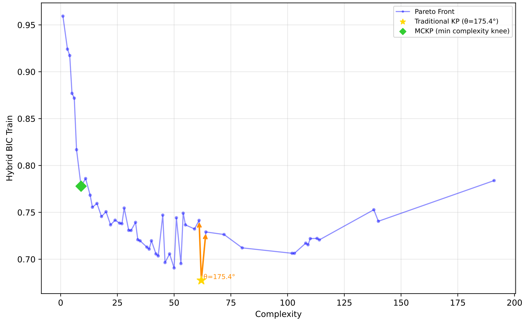
1096_FacultySalaries - Run 20 - MVP - Hybrid BIC Train \lambda_1=0.10, \lambda_2=0.00, \lambda_3=0.00 | Difficulty: 0.41 | Method: mckp
