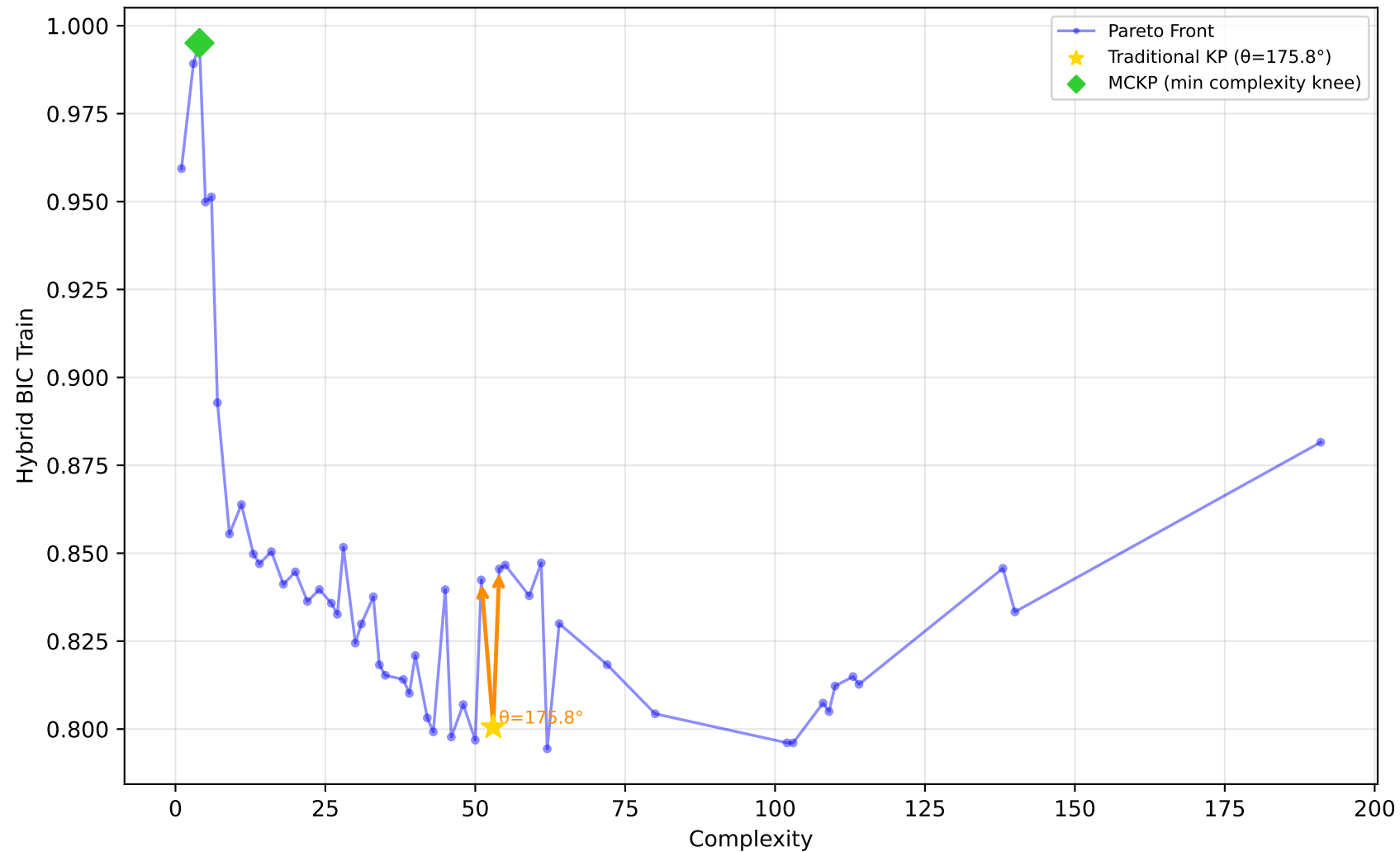
1096_FacultySalaries - Run 20 - MVP - Hybrid BIC Train \lambda_1=1.00, \lambda_2=0.00, \lambda_3=0.00 | Difficulty: 0.41 | Method: mckp
