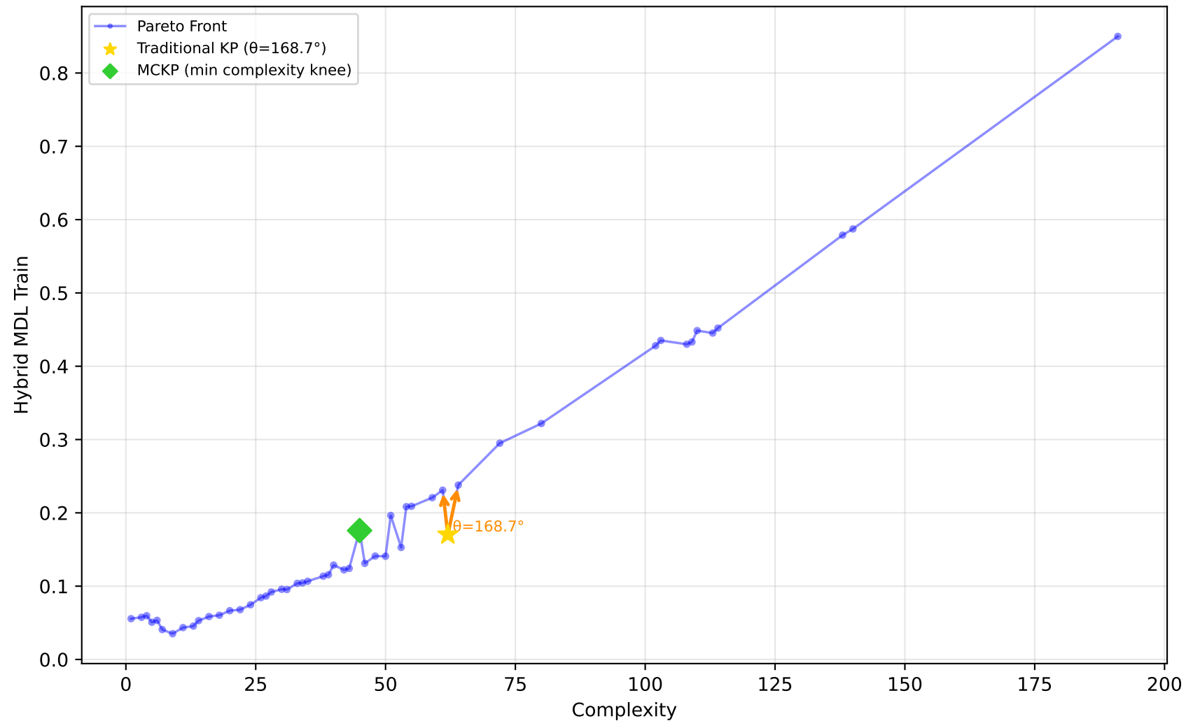
1096_FacultySalaries - Run 20 - MVP - Hybrid MDL Train \lambda_1=0.10, \lambda_2=0.00, \lambda_3=0.00 | Difficulty: 0.41 | Method: mckp
