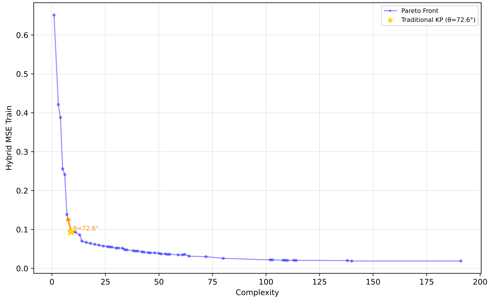
1096_FacultySalaries - Run 20 - MVP - Hybrid MSE Train \lambda_1=0.10 , \lambda_2=0.00 , \lambda_3=0.00 | Difficulty: 0.41 | Method: mckp
