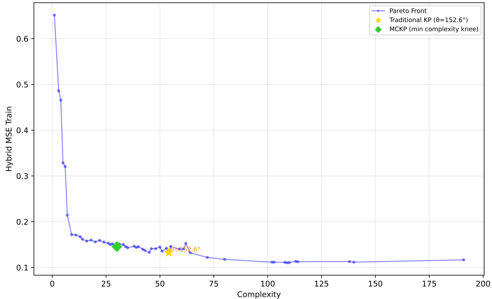
1096_FacultySalaries - Run 20 - MVP - Hybrid MSE Train \lambda_1=1.00, \lambda_2=0.00, \lambda_3=0.00 | Difficulty: 0.41 | Method: mckp
