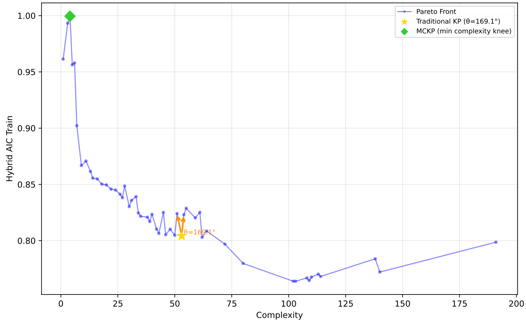
1096_FacultySalaries - Run 20 - SVP - Hybrid AIC Train \lambda_1=1.00, \lambda_2=0.00, \lambda_3=0.00 | Difficulty: 0.41 | Method: mckp
