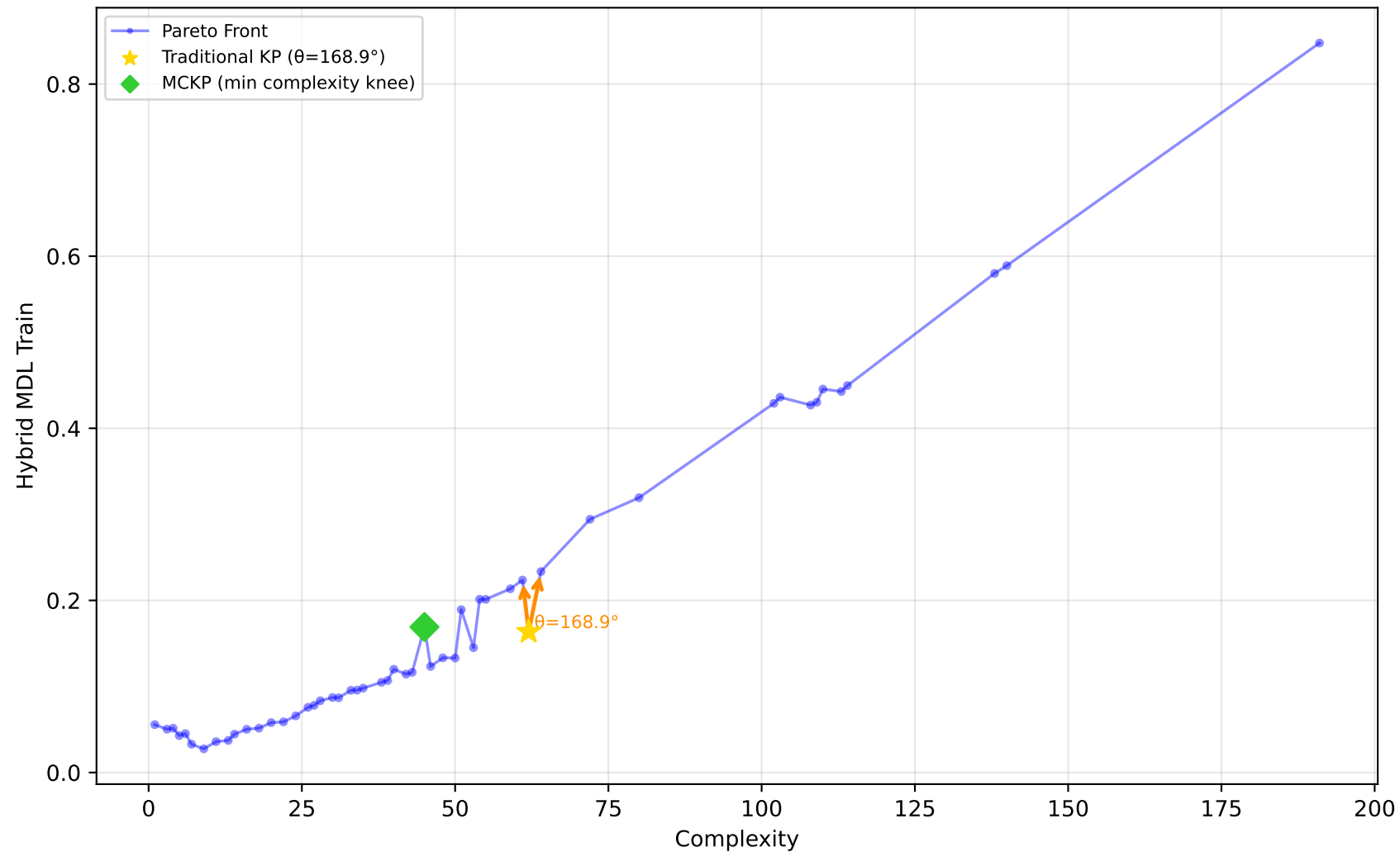
1096_FacultySalaries - Run 20 - SVP - Hybrid MDL Train \lambda_1=0.00, \lambda_2=0.90, \lambda_3=0.00 | Difficulty: 0.41 | Method: mckp
