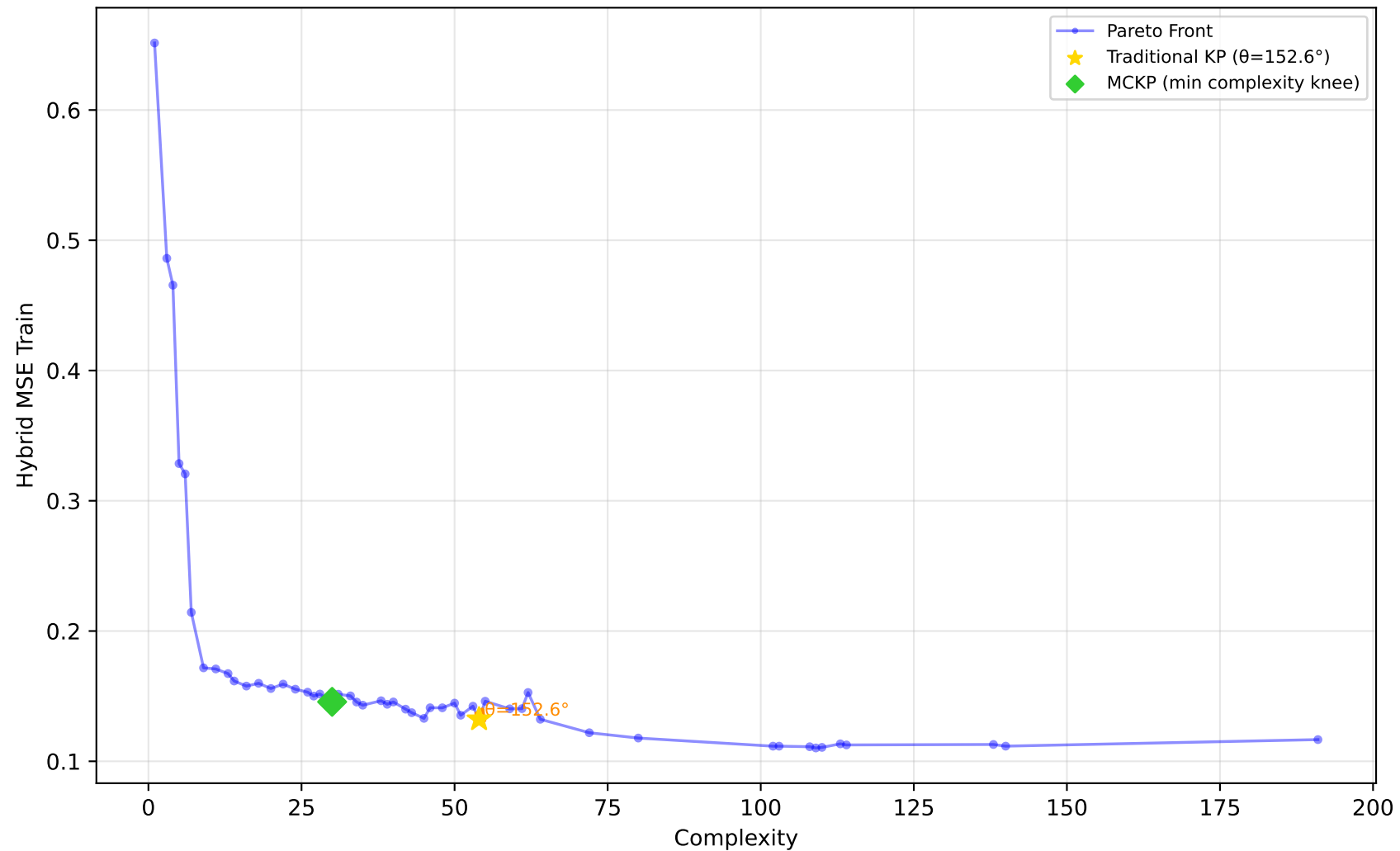
1096_FacultySalaries - Run 20 - SVP - Hybrid MSE Train \lambda_1=1.00 , \lambda_2=0.00 , \lambda_3=0.00 | Difficulty: 0.41 | Method: mckp
