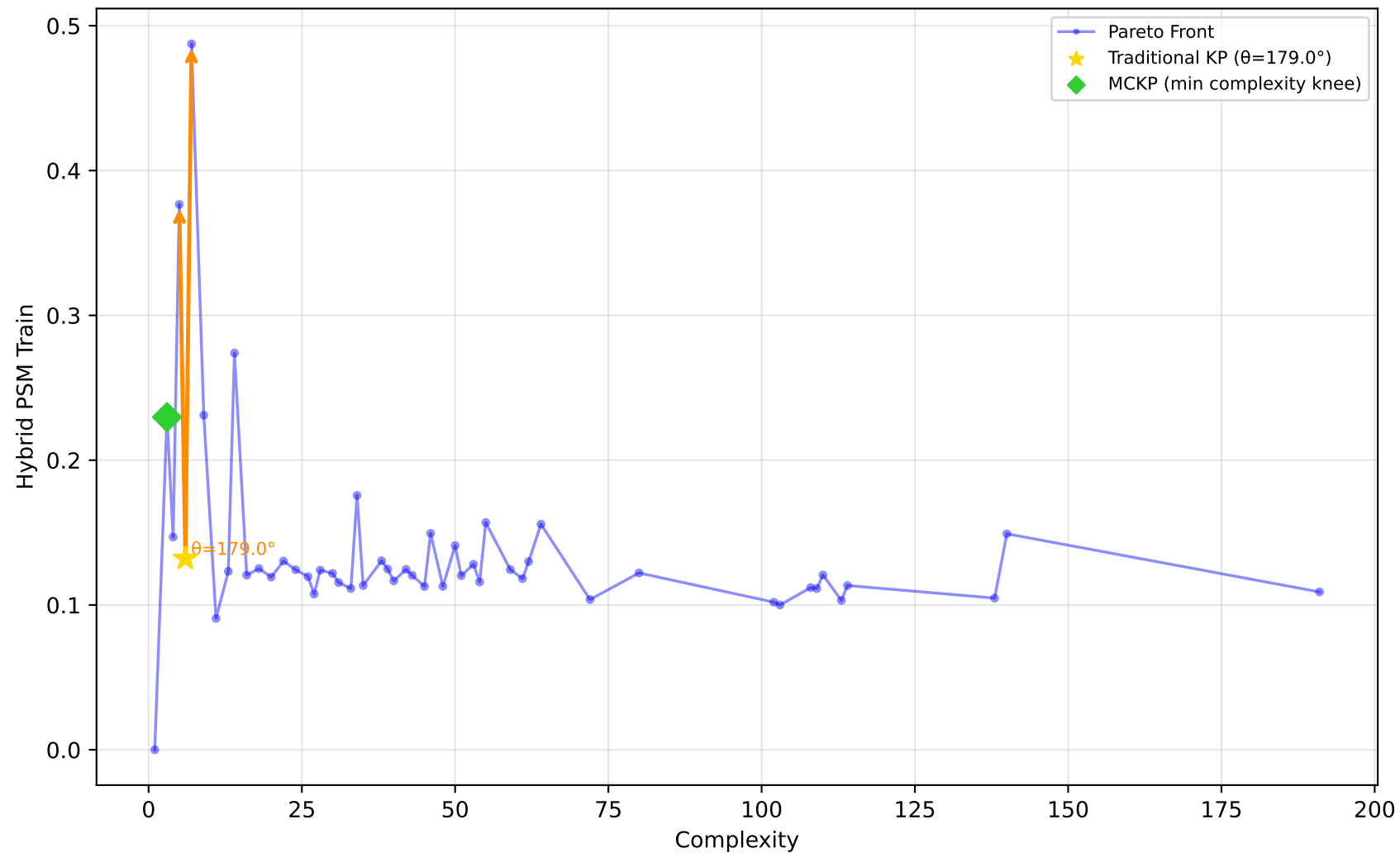
1096_FacultySalaries - Run 20 - SVP - Hybrid PSM Train \lambda_1=1.00 , \lambda_2=0.00 , \lambda_3=0.00 | Difficulty: 0.41 | Method: mckp
