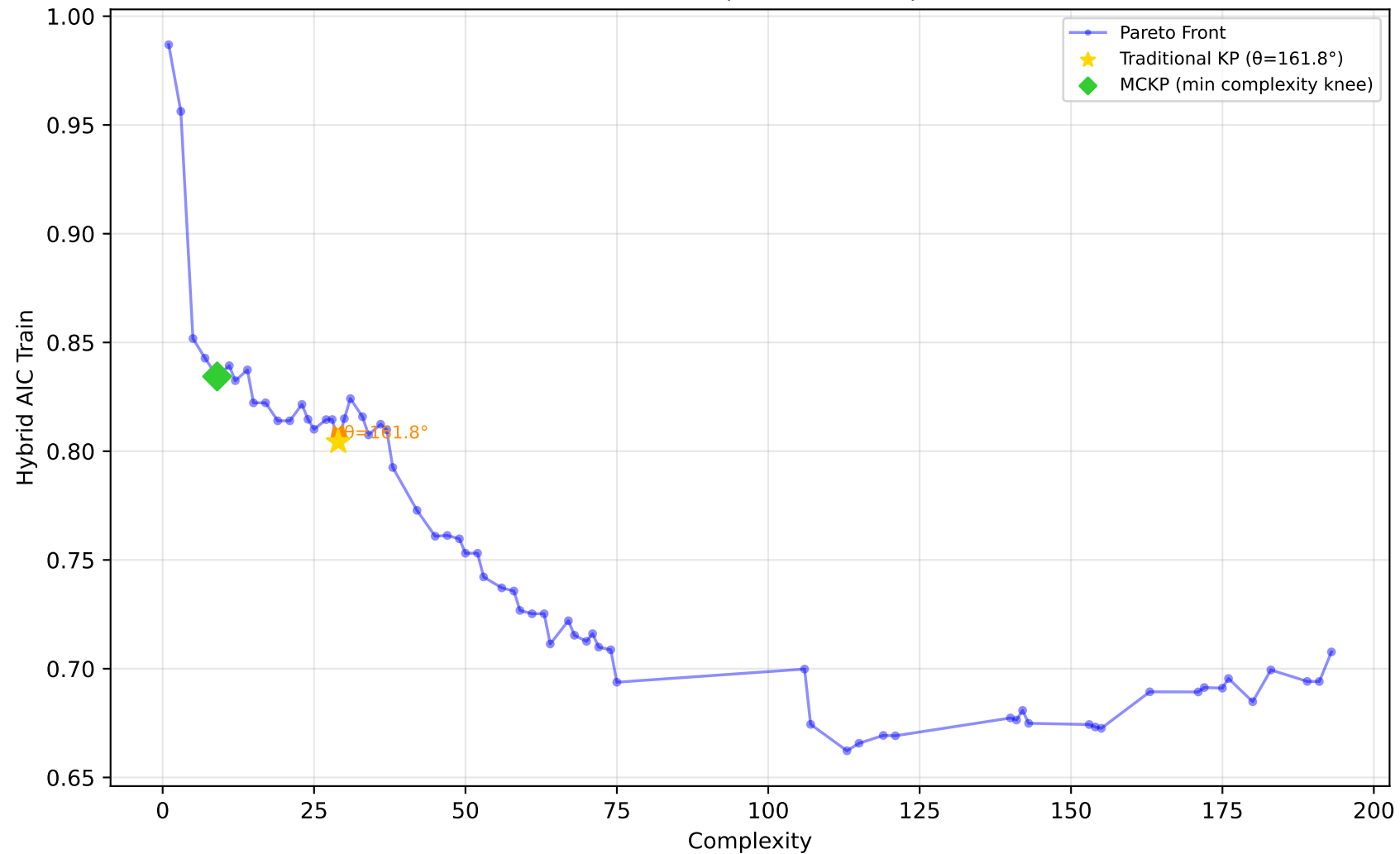
1096_FacultySalaries - Run 21 - MVP - Hybrid AIC Train \lambda_1=0.10, \lambda_2=0.00, \lambda_3=0.00 | Difficulty: 0.30 | Method: mckp
