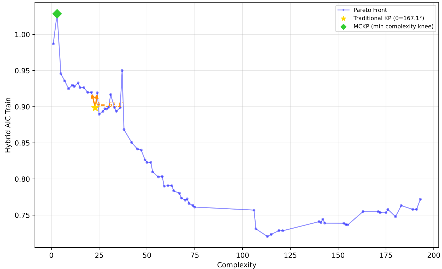
1096_FacultySalaries - Run 21 - MVP - Hybrid AIC Train \lambda_1=1.00, \lambda_2=0.00, \lambda_3=0.00 | Difficulty: 0.30 | Method: mckp
