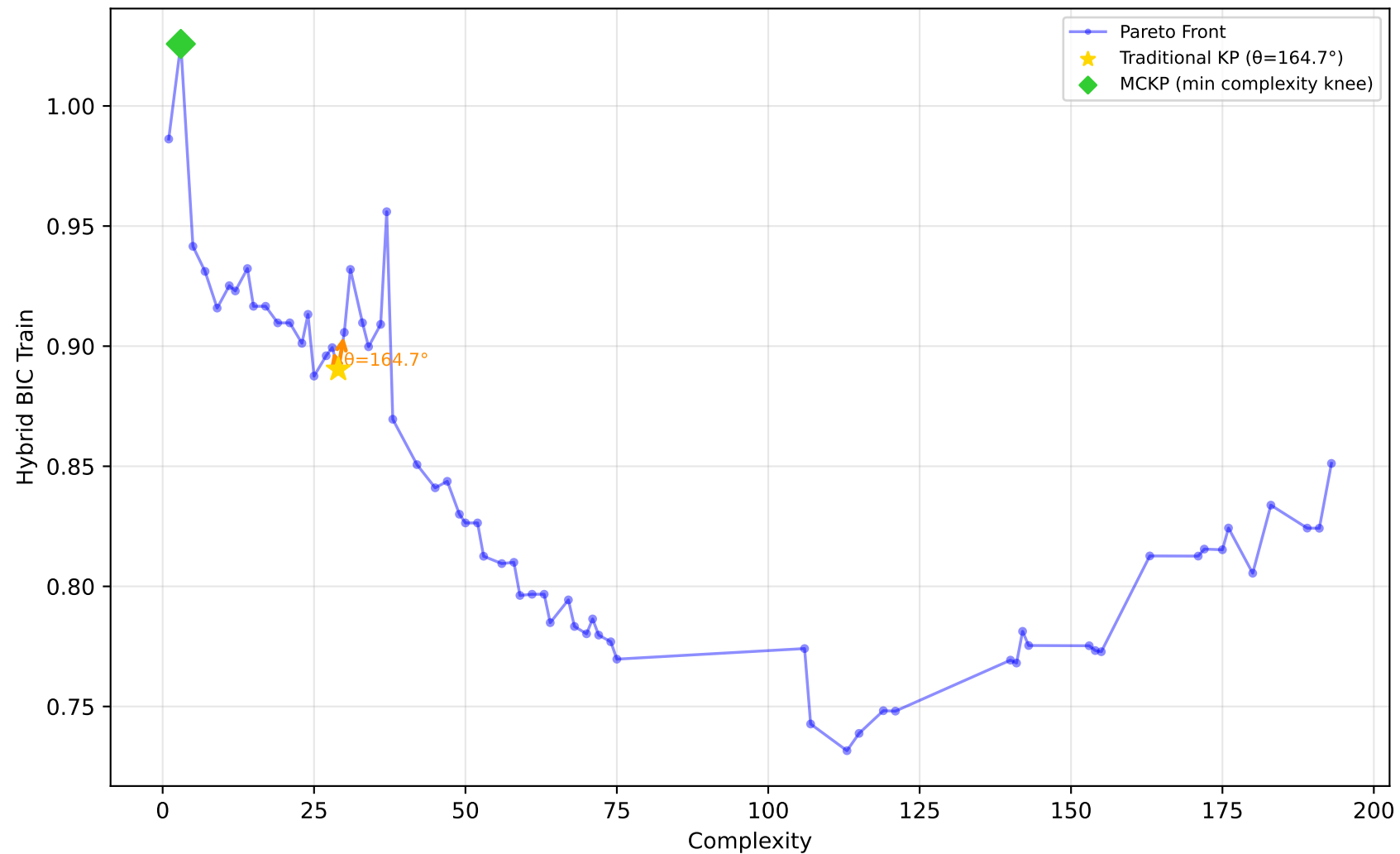
1096_FacultySalaries - Run 21 - MVP - Hybrid BIC Train \lambda_1=1.00, \lambda_2=0.00, \lambda_3=0.00 | Difficulty: 0.30 | Method: mckp
