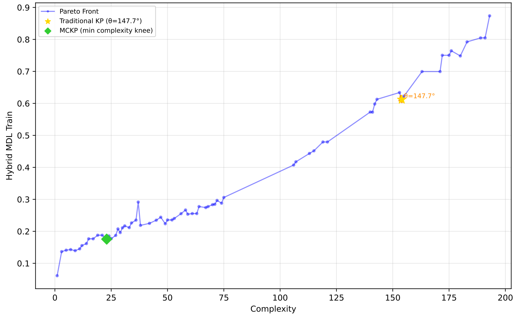
1096_FacultySalaries - Run 21 - MVP - Hybrid MDL Train \lambda_1=1.00 , \lambda_2=0.00 , \lambda_3=0.00 | Difficulty: 0.30 | Method: mckp
