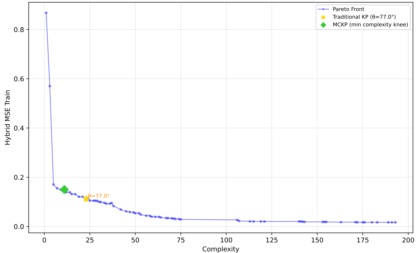
1096_FacultySalaries - Run 21 - MVP - Hybrid MSE Train \lambda_1=0.10 , \lambda_2=0.00 , \lambda_3=0.00 | Difficulty: 0.30 | Method: mckp
