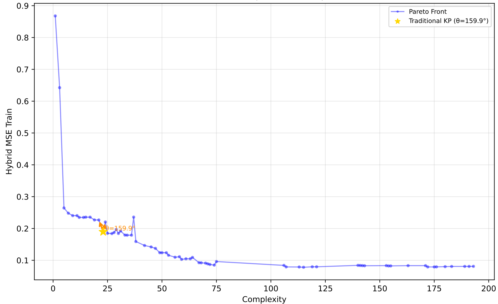
1096_FacultySalaries - Run 21 - MVP - Hybrid MSE Train \lambda_1=1.00 , \lambda_2=0.00 , \lambda_3=0.00 | Difficulty: 0.30 | Method: mckp
