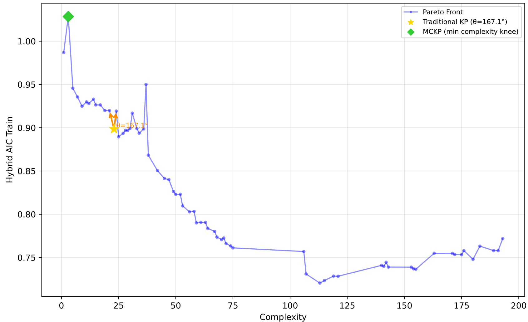
1096_FacultySalaries - Run 21 - SVP - Hybrid AIC Train \lambda_1=1.00, \lambda_2=0.00, \lambda_3=0.00 | Difficulty: 0.30 | Method: mckp
