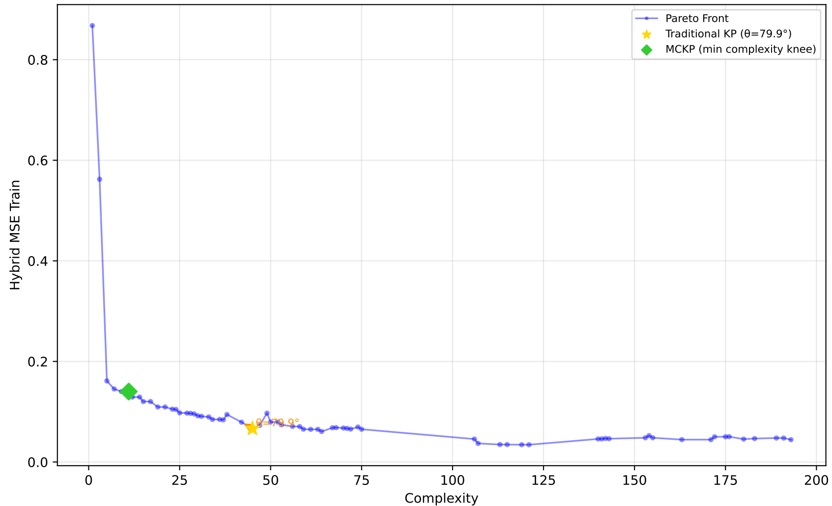
1096_FacultySalaries - Run 21 - SVP - Hybrid MSE Train \lambda_1=0.00 , \lambda_2=0.90 , \lambda_3=0.00 | Difficulty: 0.30 | Method: mckp
