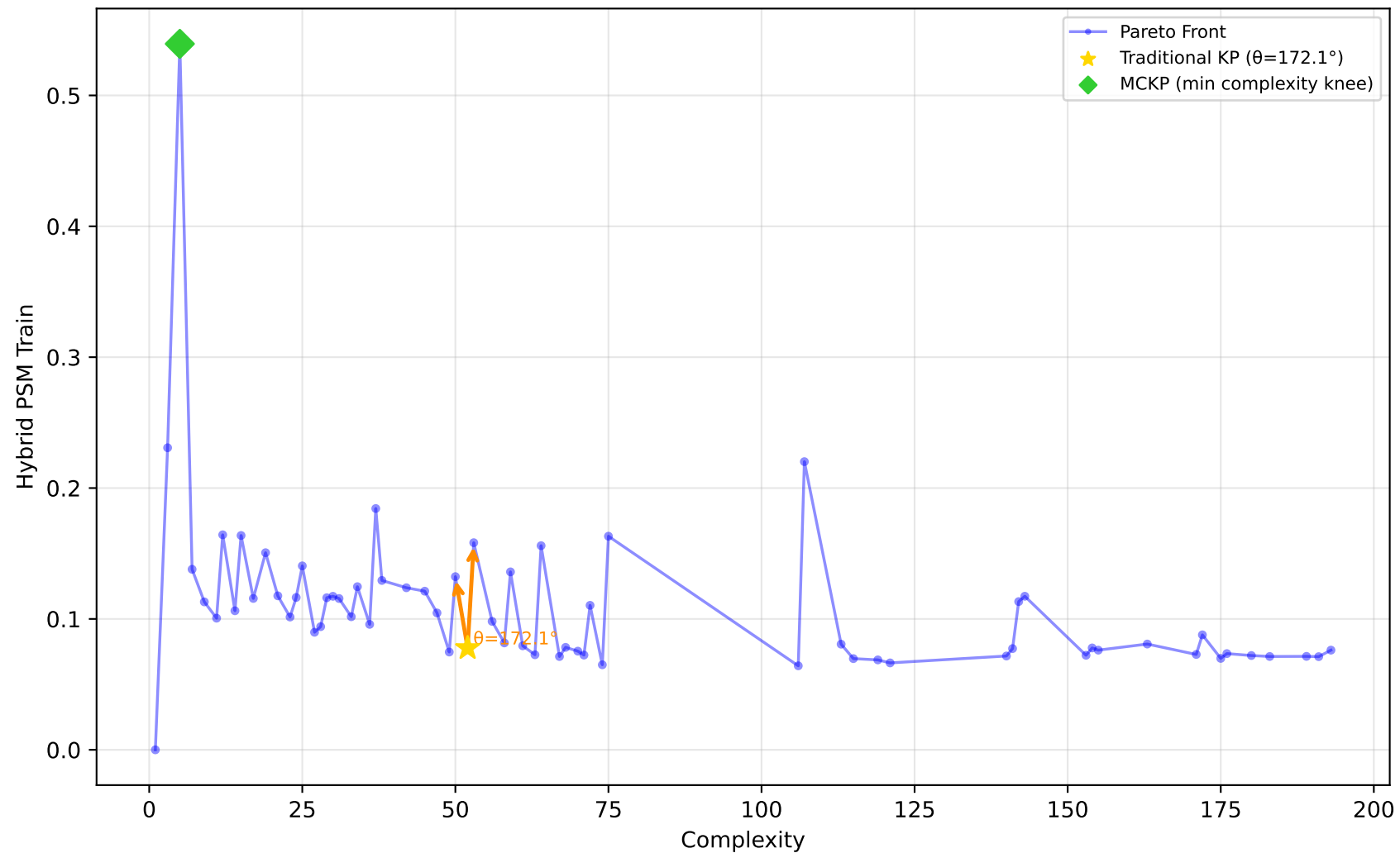
1096_FacultySalaries - Run 21 - SVP - Hybrid PSM Train \lambda_1=1.00 , \lambda_2=0.00 , \lambda_3=0.00 | Difficulty: 0.30 | Method: mckp
