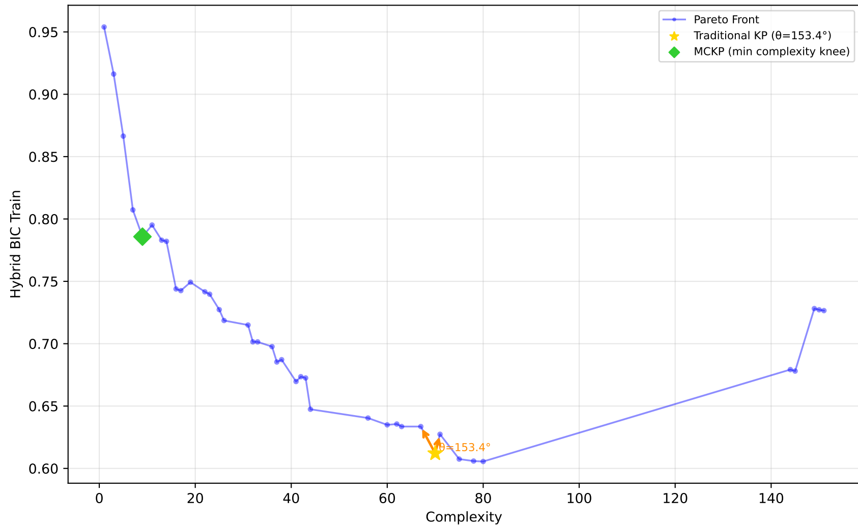
1096_FacultySalaries - Run 22 - MVP - Hybrid BIC Train \lambda_1=0.10 , \lambda_2=0.00 , \lambda_3=0.00 | Difficulty: 1.00 | Method: hmr
