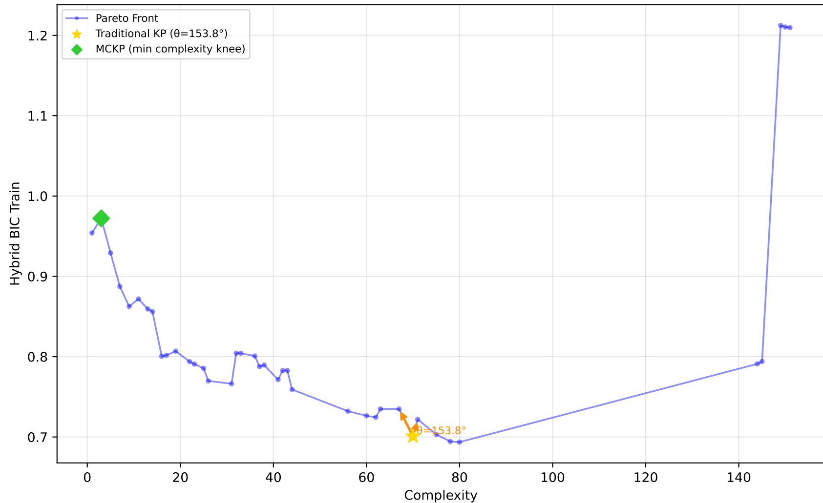
1096_FacultySalaries - Run 22 - MVP - Hybrid BIC Train \lambda_1=1.00 , \lambda_2=0.00 , \lambda_3=0.00 | Difficulty: 1.00 | Method: hmr
