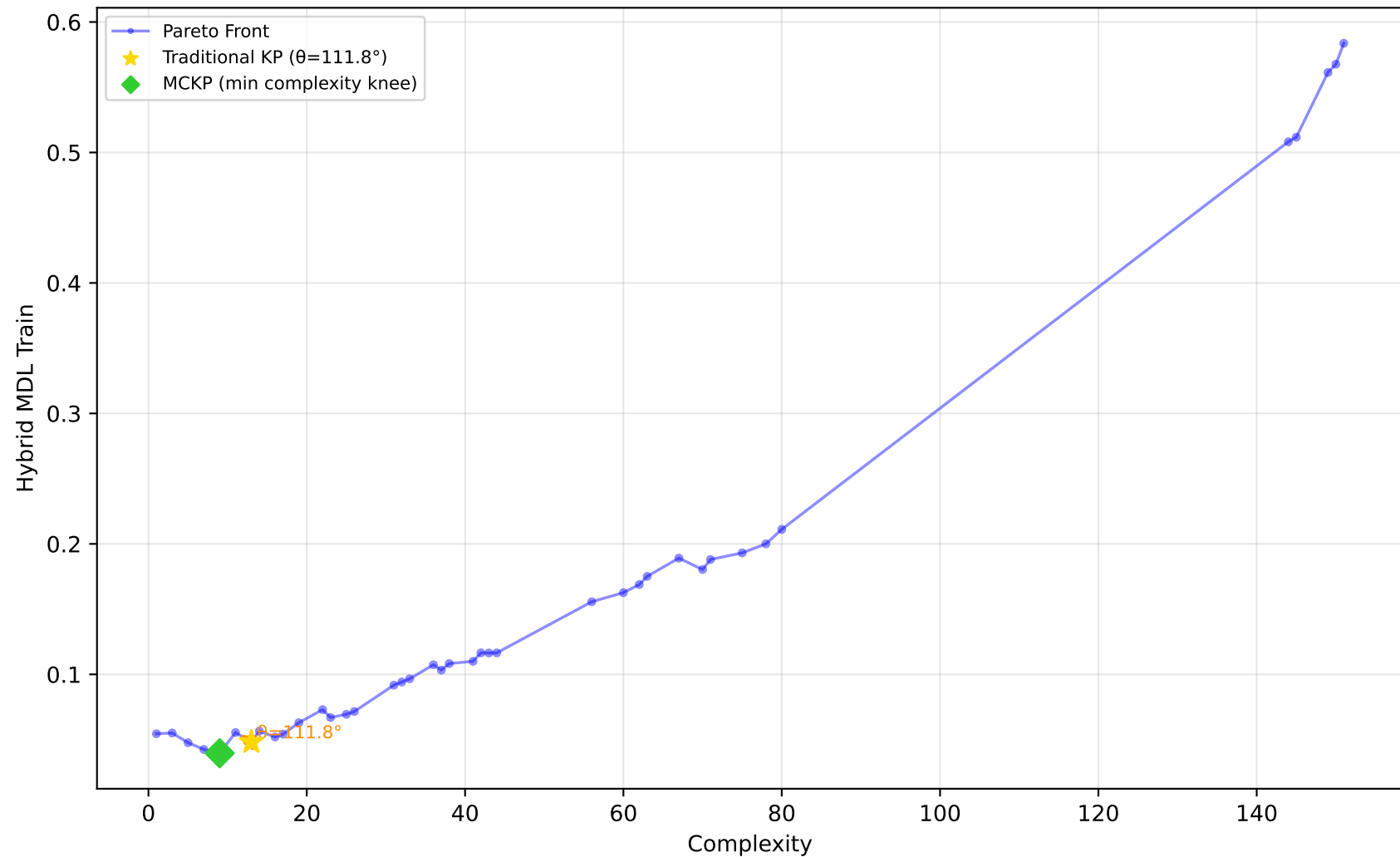
1096_FacultySalaries - Run 22 - MVP - Hybrid MDL Train \lambda_1=0.10, \lambda_2=0.00, \lambda_3=0.00 | Difficulty: 1.00 | Method: hmr
