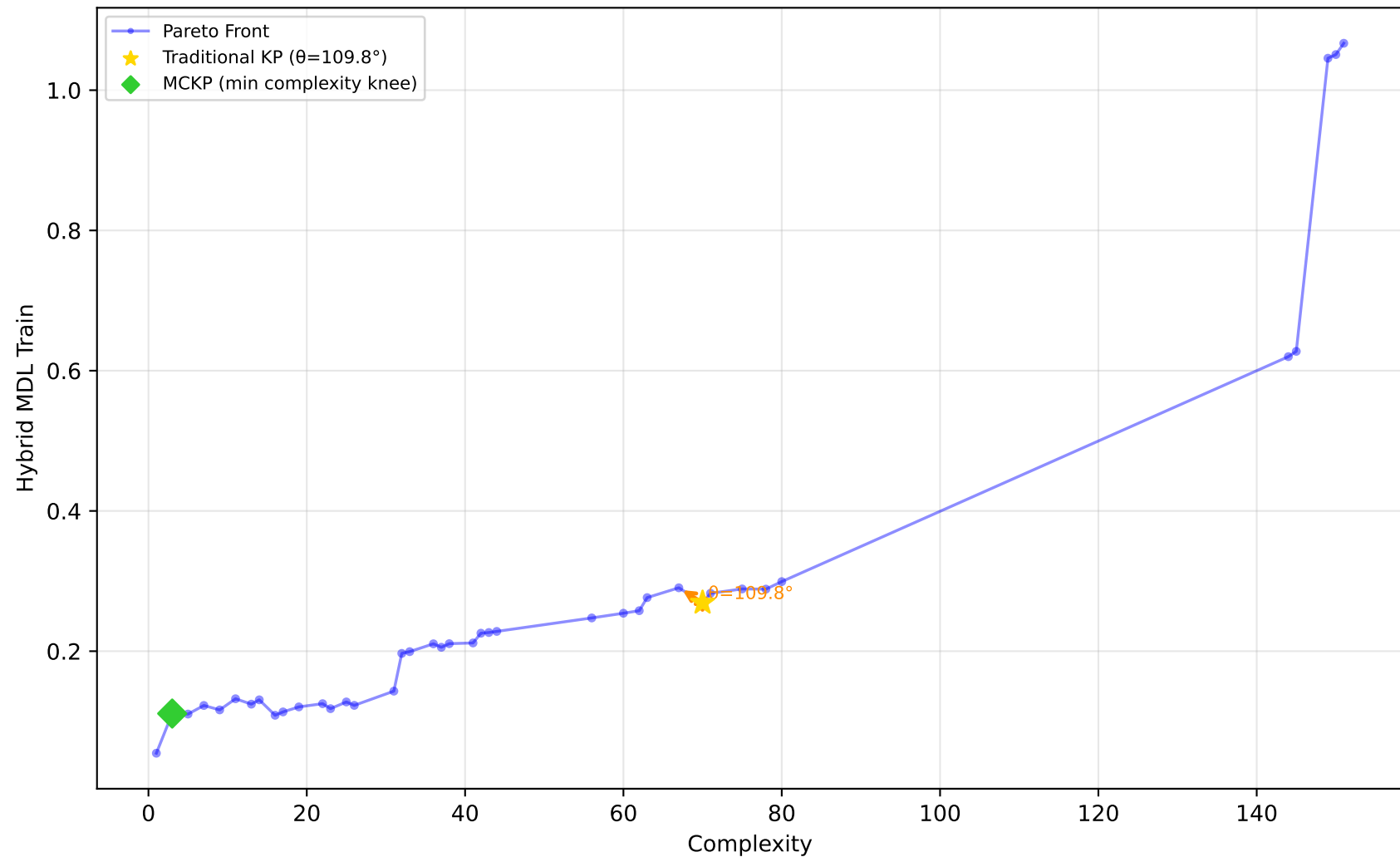
1096_FacultySalaries - Run 22 - MVP - Hybrid MDL Train \lambda_1=1.00, \lambda_2=0.00, \lambda_3=0.00 | Difficulty: 1.00 | Method: hmr
