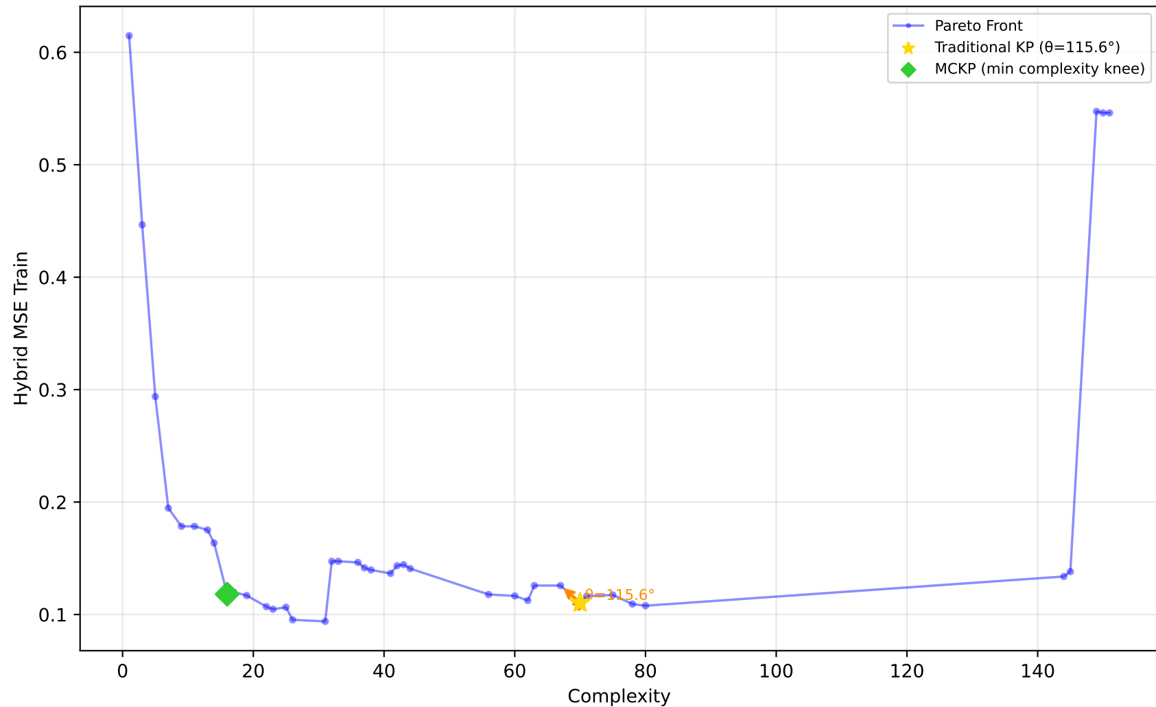
1096_FacultySalaries - Run 22 - MVP - Hybrid MSE Train \lambda_1=1.00, \lambda_2=0.00, \lambda_3=0.00 | Difficulty: 1.00 | Method: hmr
