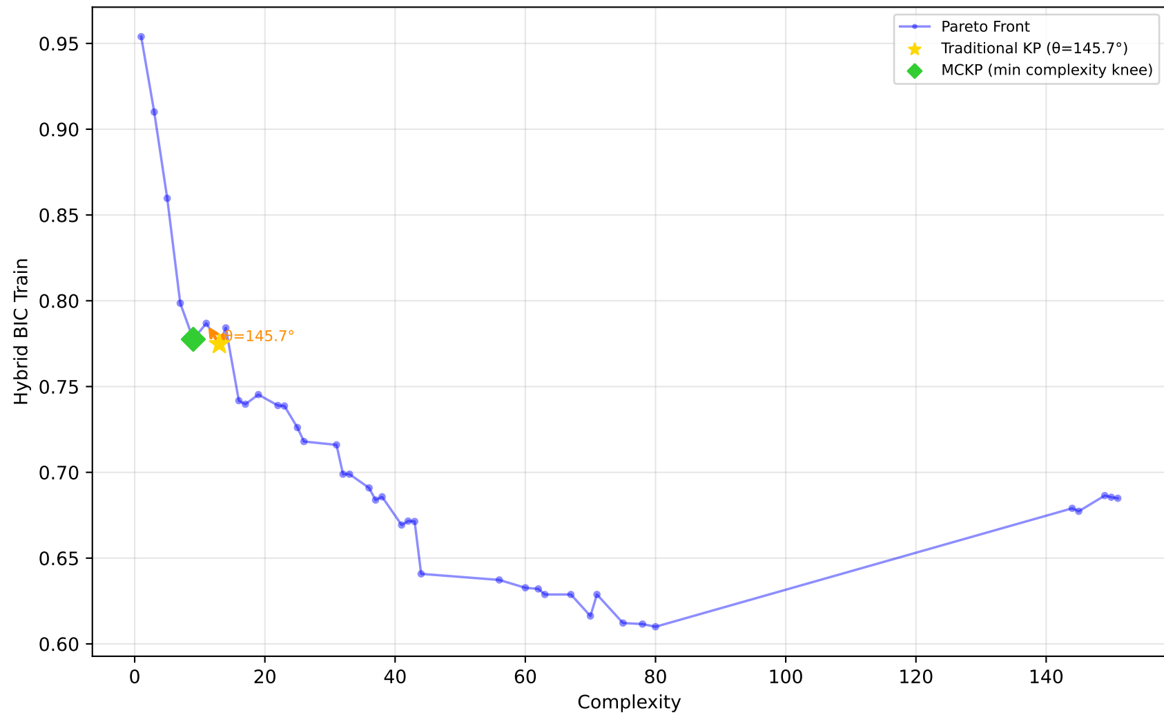
1096_FacultySalaries - Run 22 - SVP - Hybrid BIC Train \lambda_1=0.00 , \lambda_2=0.90 , \lambda_3=0.00 | Difficulty: 1.00 | Method: hmr
