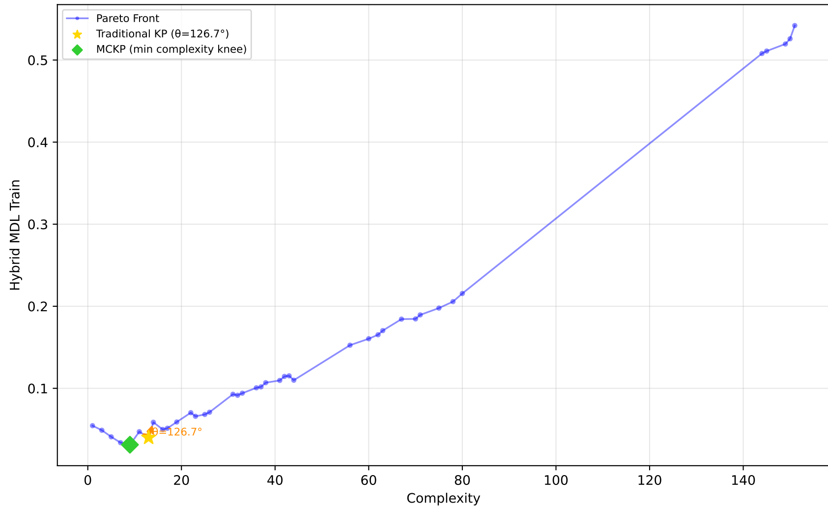
1096_FacultySalaries - Run 22 - SVP - Hybrid MDL Train \lambda_1=0.00 , \lambda_2=0.90 , \lambda_3=0.00 | Difficulty: 1.00 | Method: hmr
