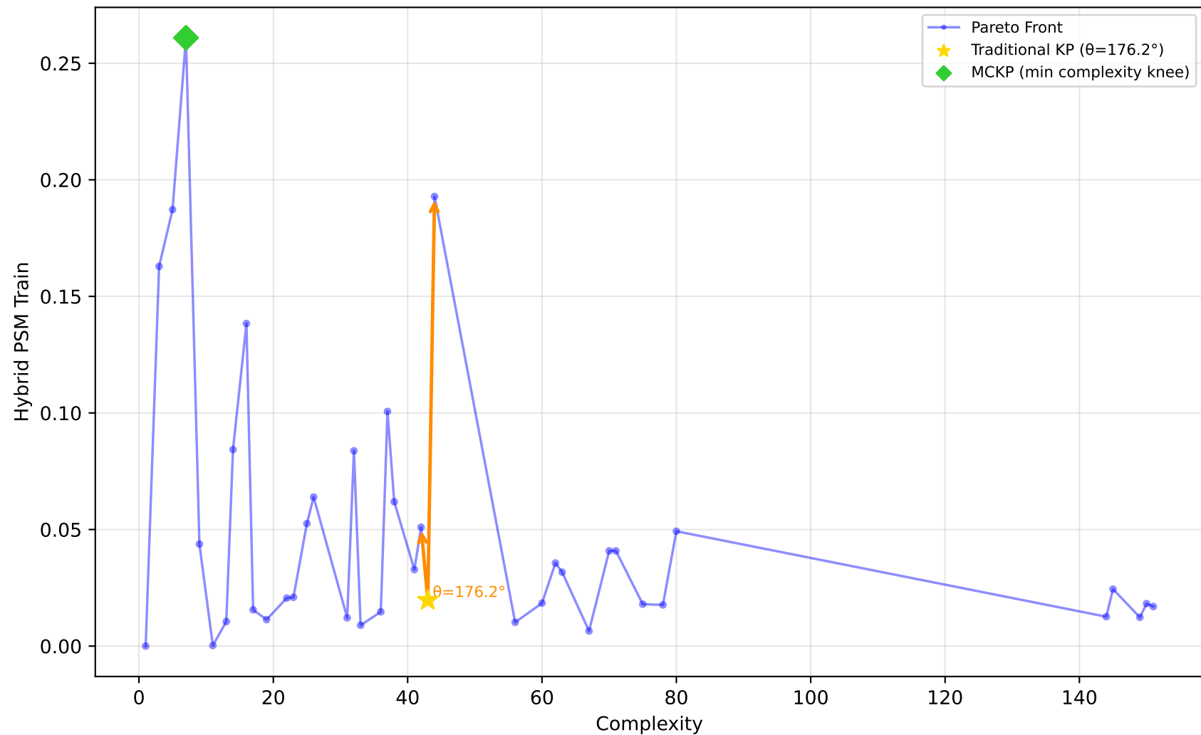
1096_FacultySalaries - Run 22 - SVP - Hybrid PSM Train \lambda_1=0.00 , \lambda_2=0.90 , \lambda_3=0.00 | Difficulty: 1.00 | Method: hmr
