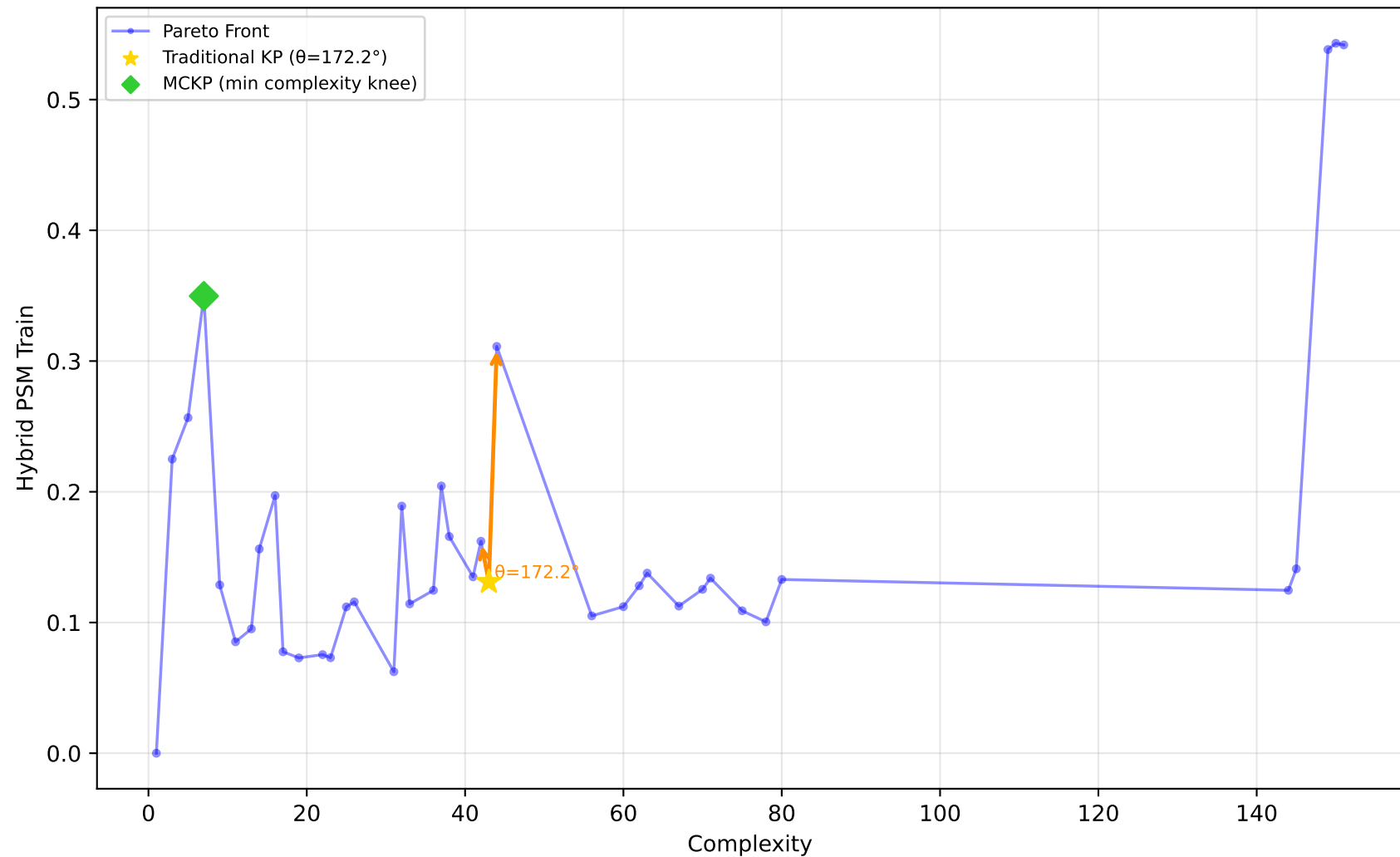
1096_FacultySalaries - Run 22 - SVP - Hybrid PSM Train \lambda_1=1.00, \lambda_2=0.00, \lambda_3=0.00 | Difficulty: 1.00 | Method: hmr
