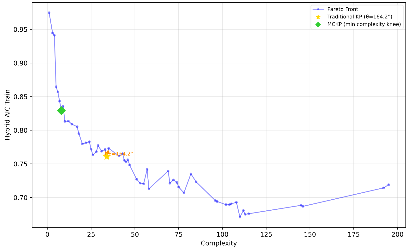
1096_FacultySalaries - Run 23 - MVP - Hybrid AIC Train \lambda_1=0.10 , \lambda_2=0.00 , \lambda_3=0.00 | Difficulty: 1.00 | Method: hmr
