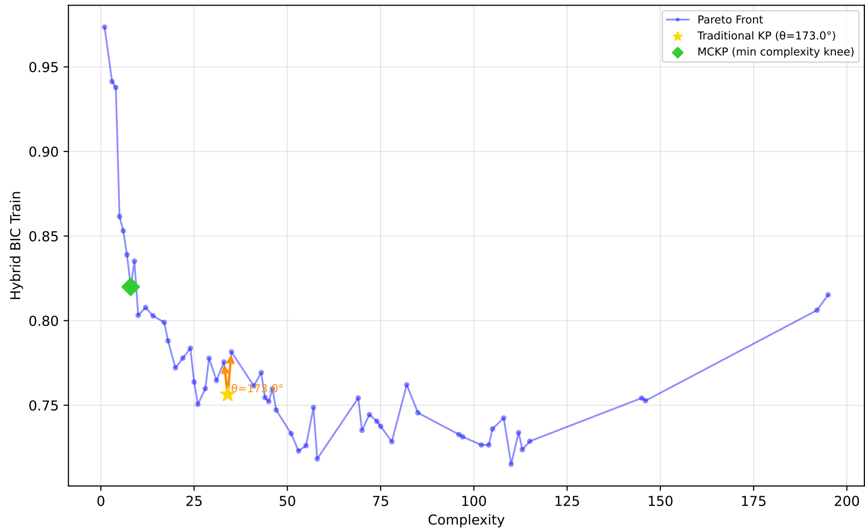
1096_FacultySalaries - Run 23 - MVP - Hybrid BIC Train \lambda_1=0.10 , \lambda_2=0.00 , \lambda_3=0.00 | Difficulty: 1.00 | Method: hmr
