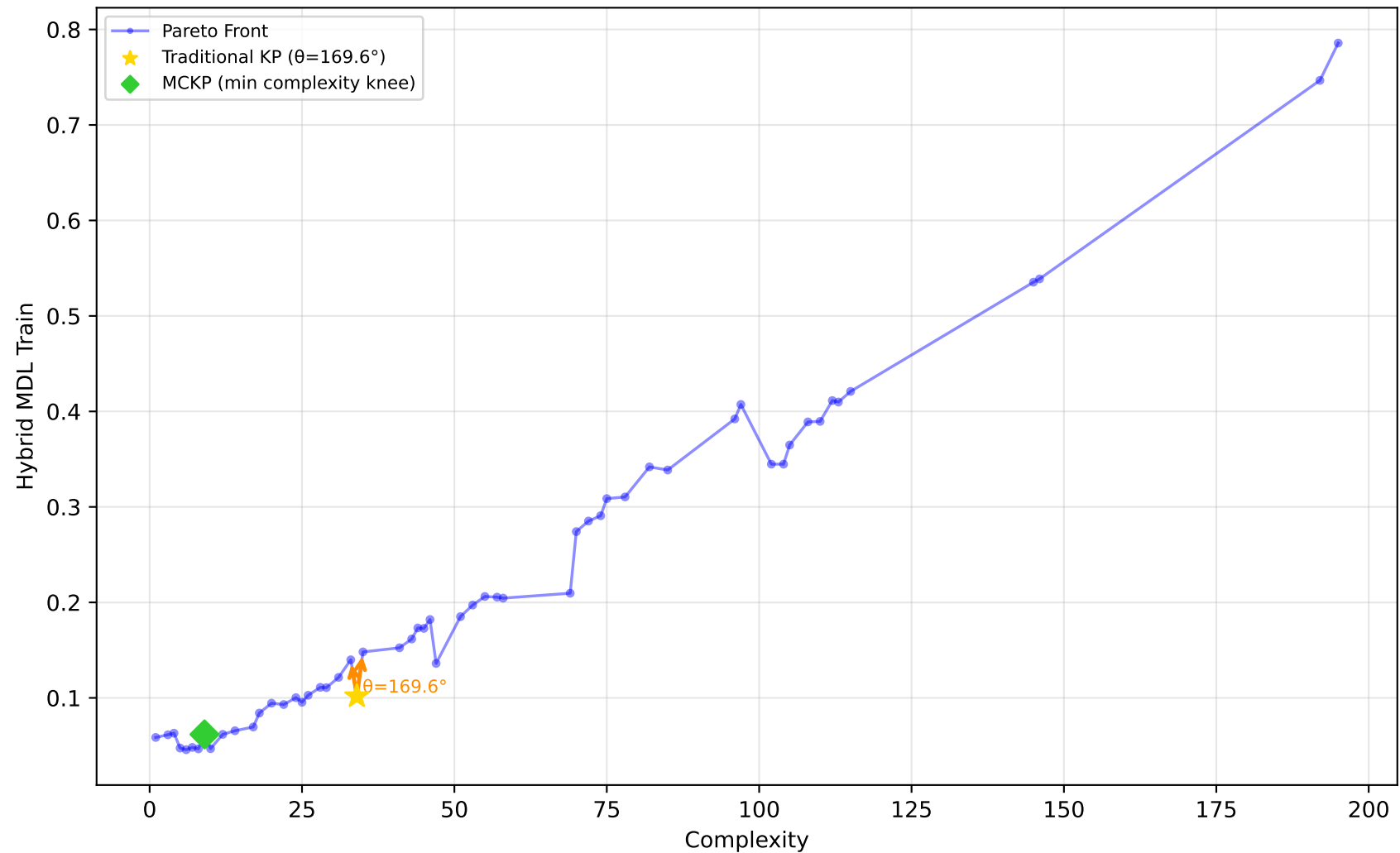
1096_FacultySalaries - Run 23 - MVP - Hybrid MDL Train \lambda_1=0.10, \lambda_2=0.00, \lambda_3=0.00 | Difficulty: 1.00 | Method: hmr
